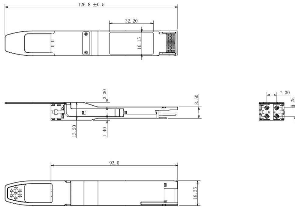
Figure5. Mechanical Specifications
