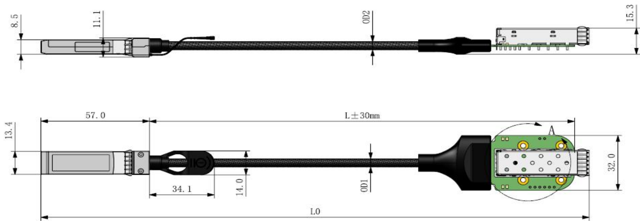
Figure 4. SFP28 extender Mechanical Specifications
