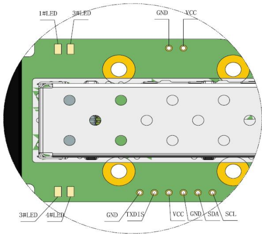
Figure 5. Extender housing pin
