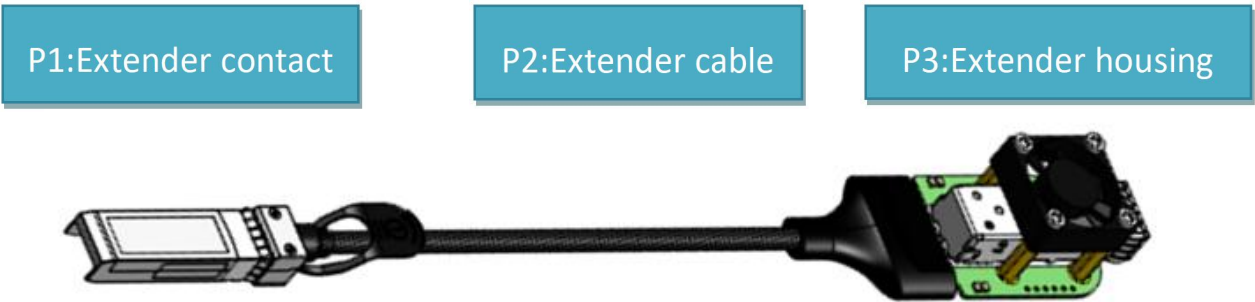
Figure 3 SFP112 extender main part assembly
