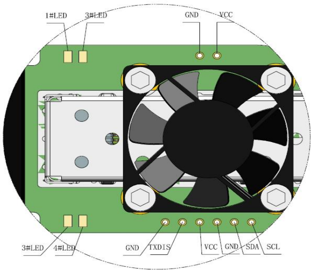
Figure 5. Extender housing pin
