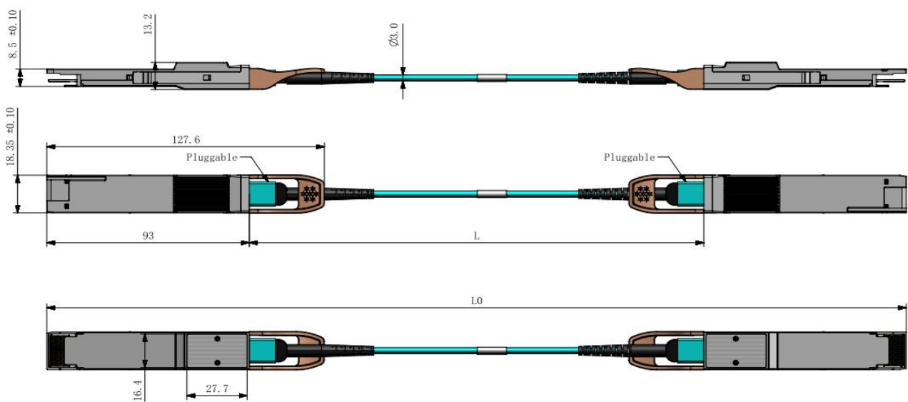
Figure7. Mechanical Specifications
