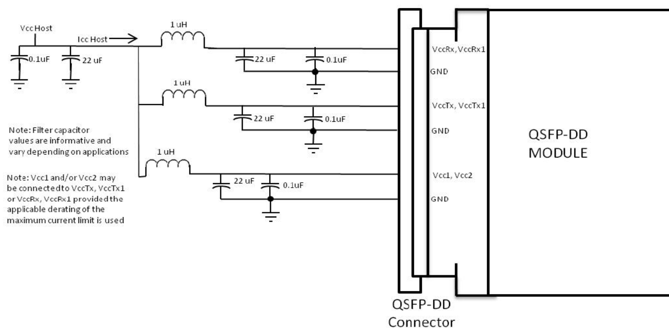
Figure4. Host Board Power Supply Filtering
