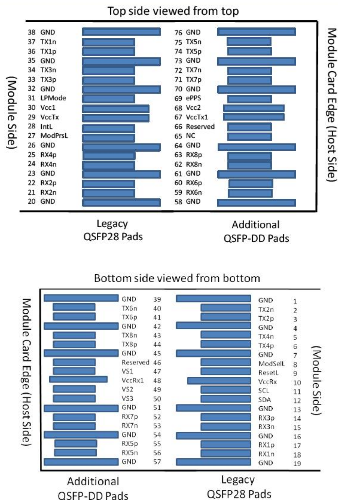
Figure3. Electrical Pin-out Details
