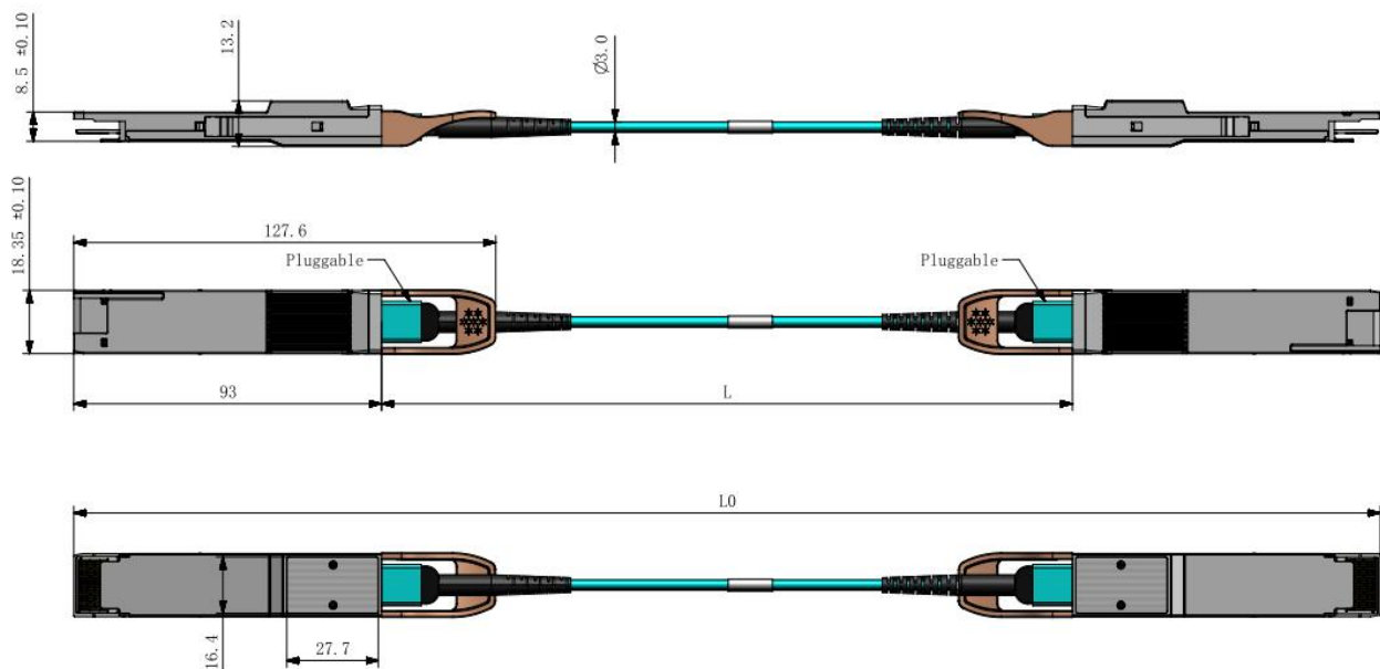
Figure7. Mechanical Specifications
