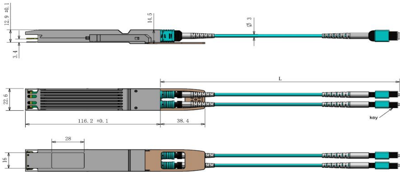
Figure7. Mechanical Specifications
