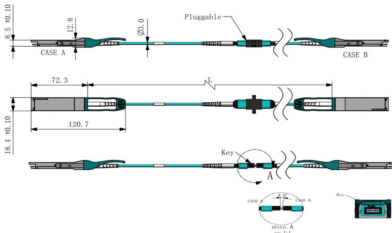
Figure 7. Mechanical Specifications
