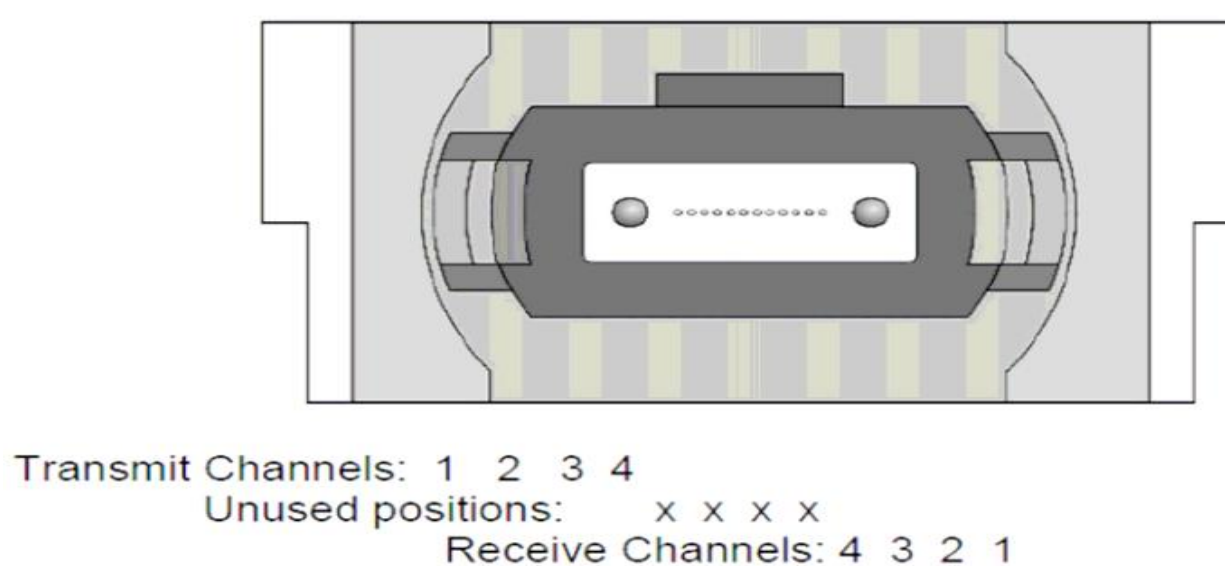
Figure 5. Optical interface and Channel Orientation
