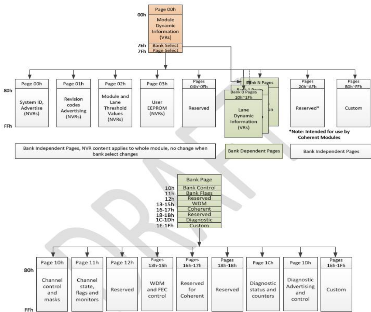
Figure 6. Memory Map
