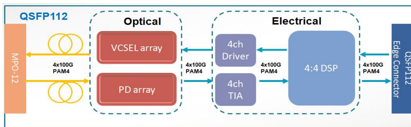
Figure1. Module Block Diagram
