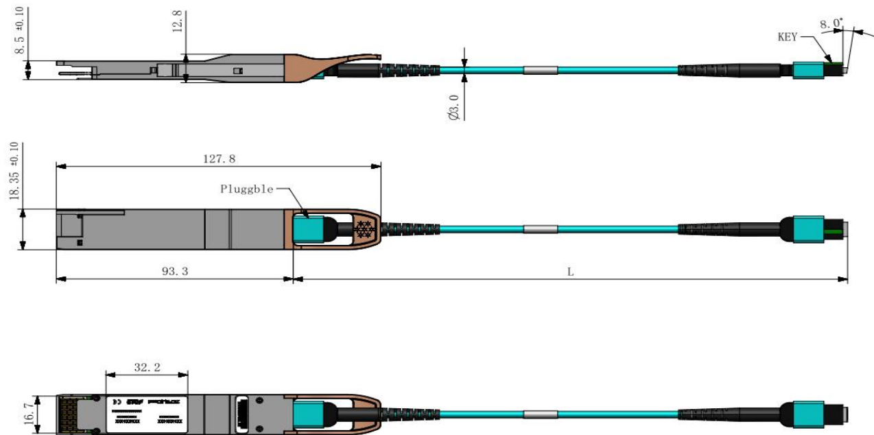
Figure7. Mechanical Specifications
