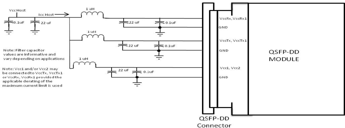
Figure4. Host Board Power Supply Filtering
