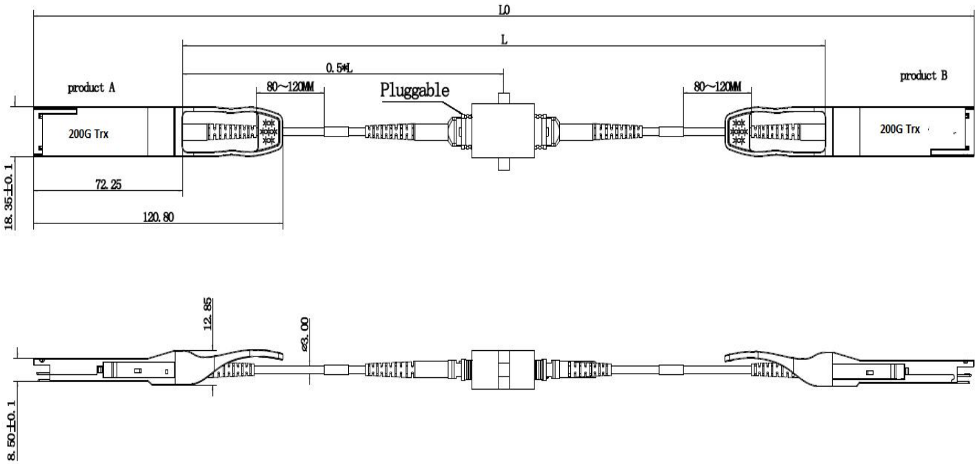
Figure 13. Mechanical Specifications
