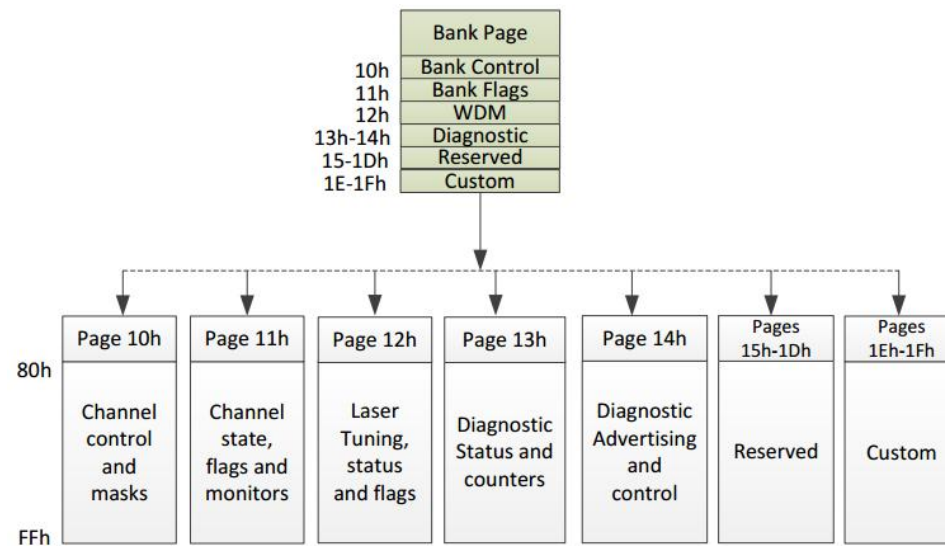
Figure 7. Additional Supported Bank Page Memory Map
