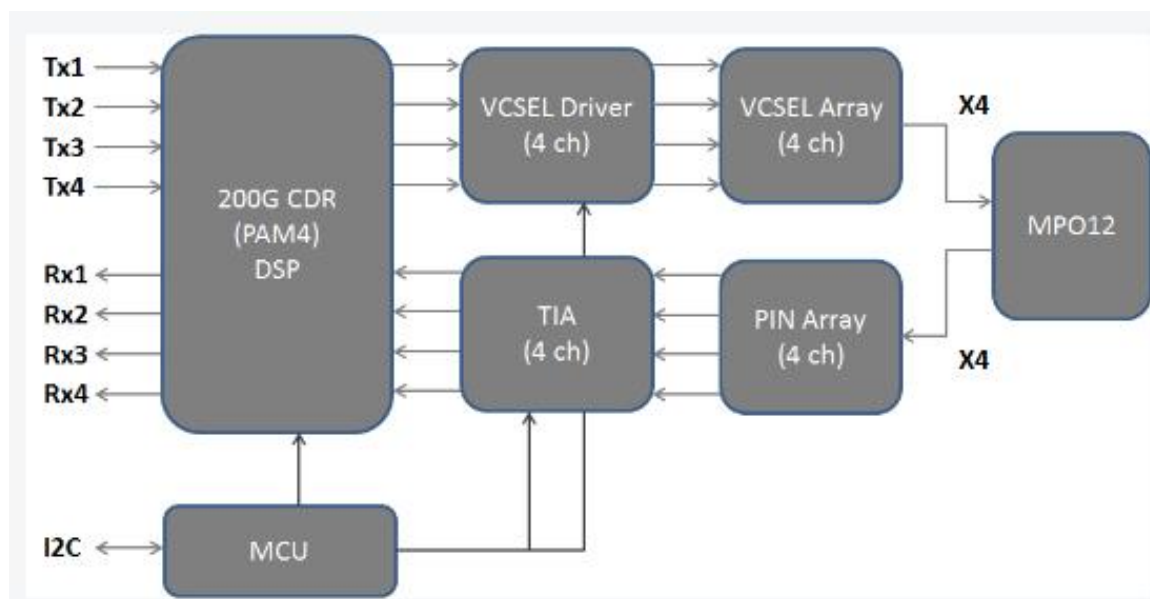
Figure 2. Module Block Diagram
