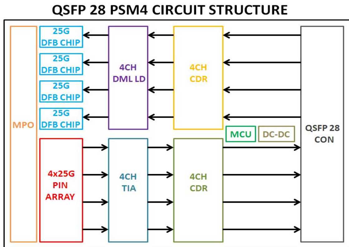
Figure2. Module Block Diagram
