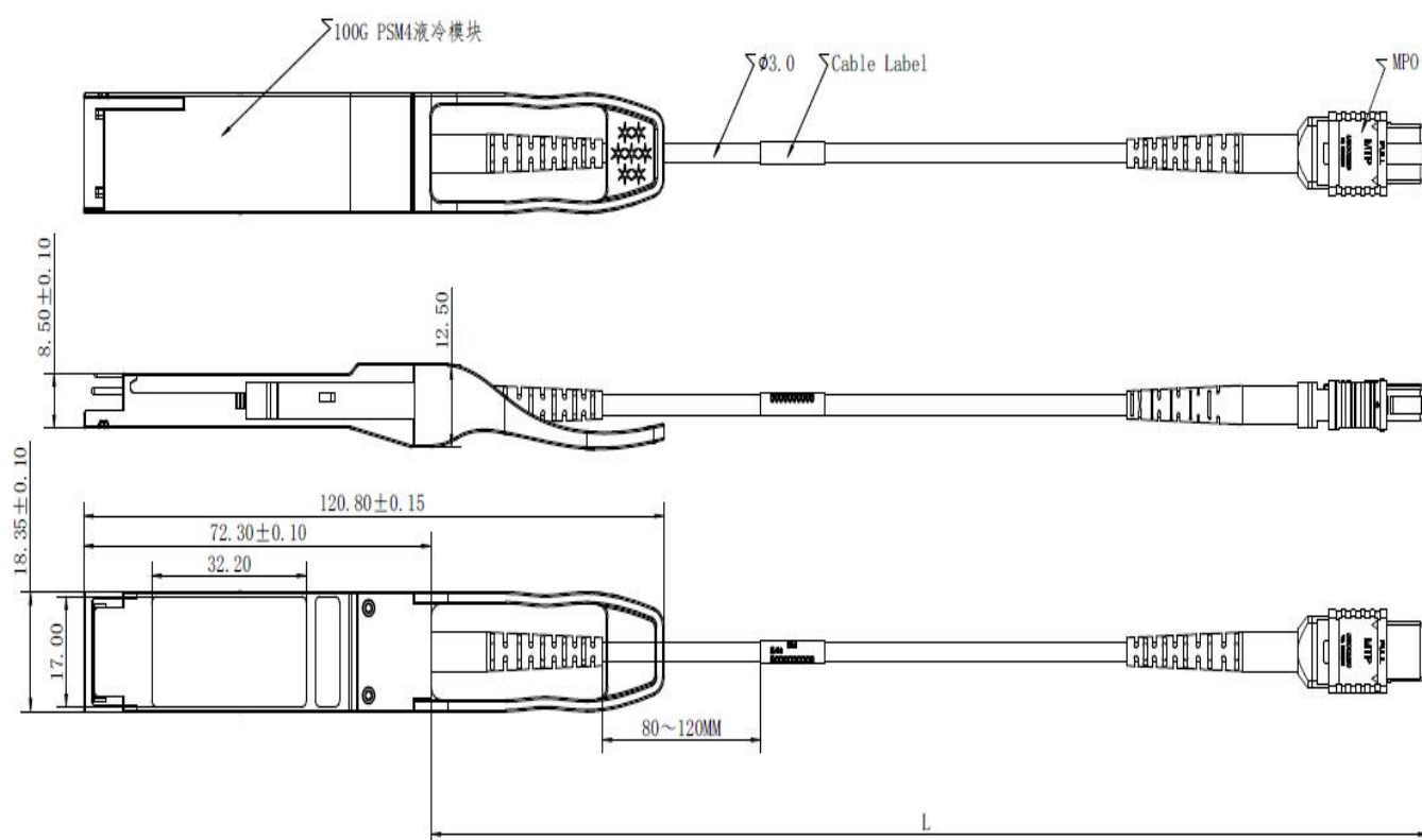
Figure9. Mechanical Specifications
