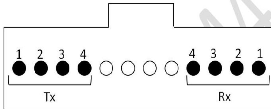
Figure 5. MPO Optical interface and Channel Orientation
