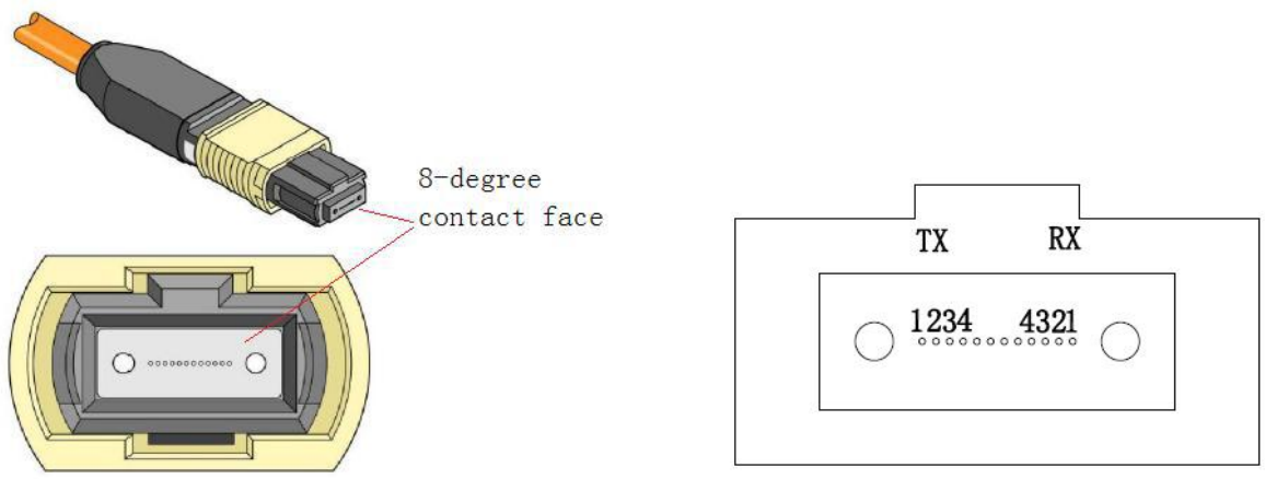
male MPO(APC 8-degree) pigtail overview
