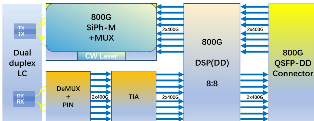
Figure1. 2xFR4 Module Block Diagram
