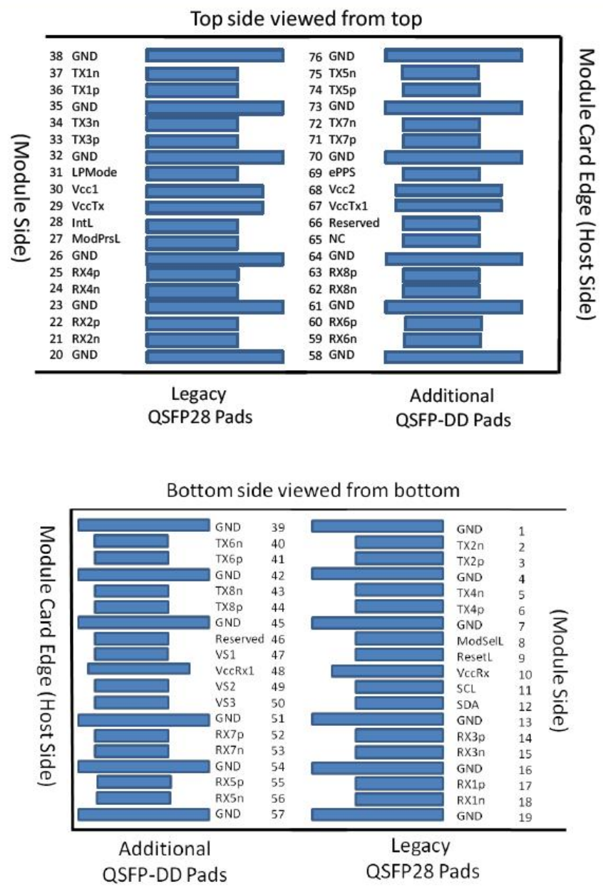
Figure2. QSFP-DD module Pin-out Details
