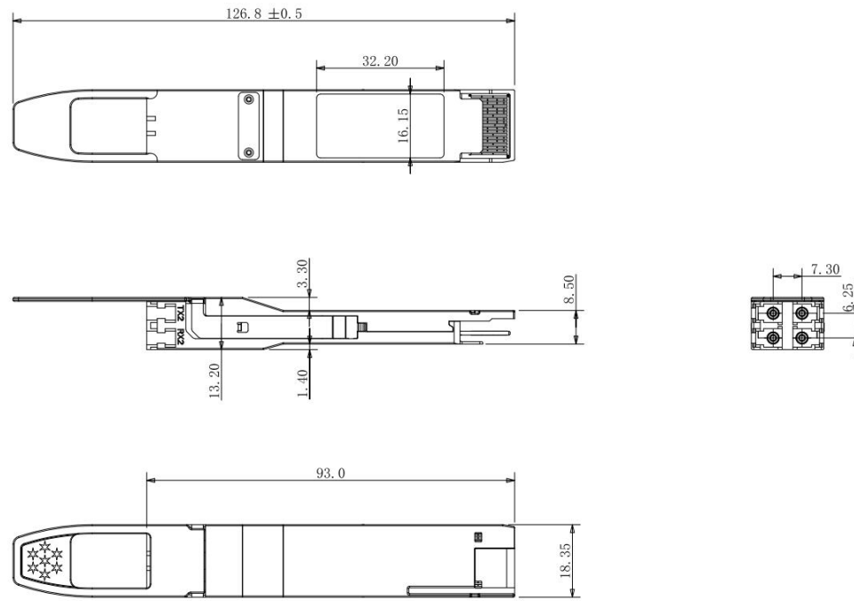
Figure5. Mechanical Specifications
