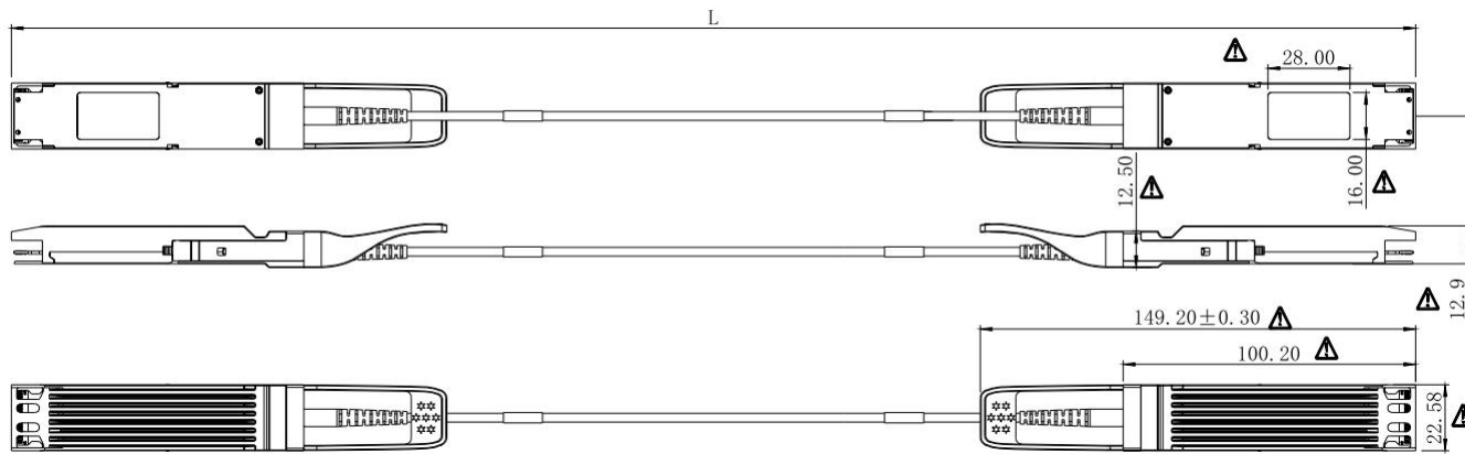
Figure5. Mechanical Specifications
