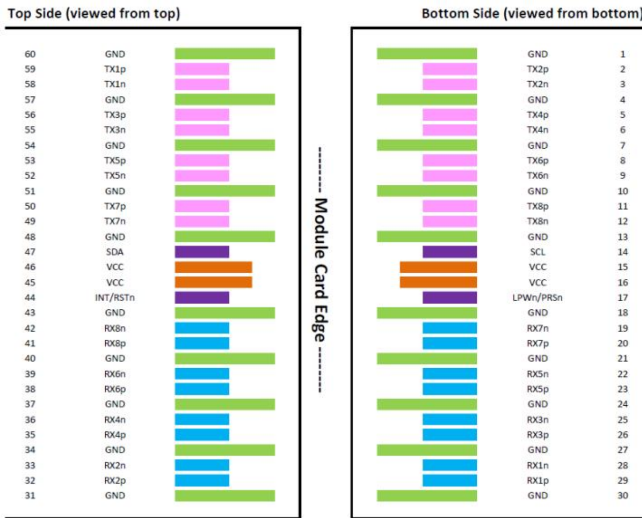
Figure2. Electrical Pin-out Details
