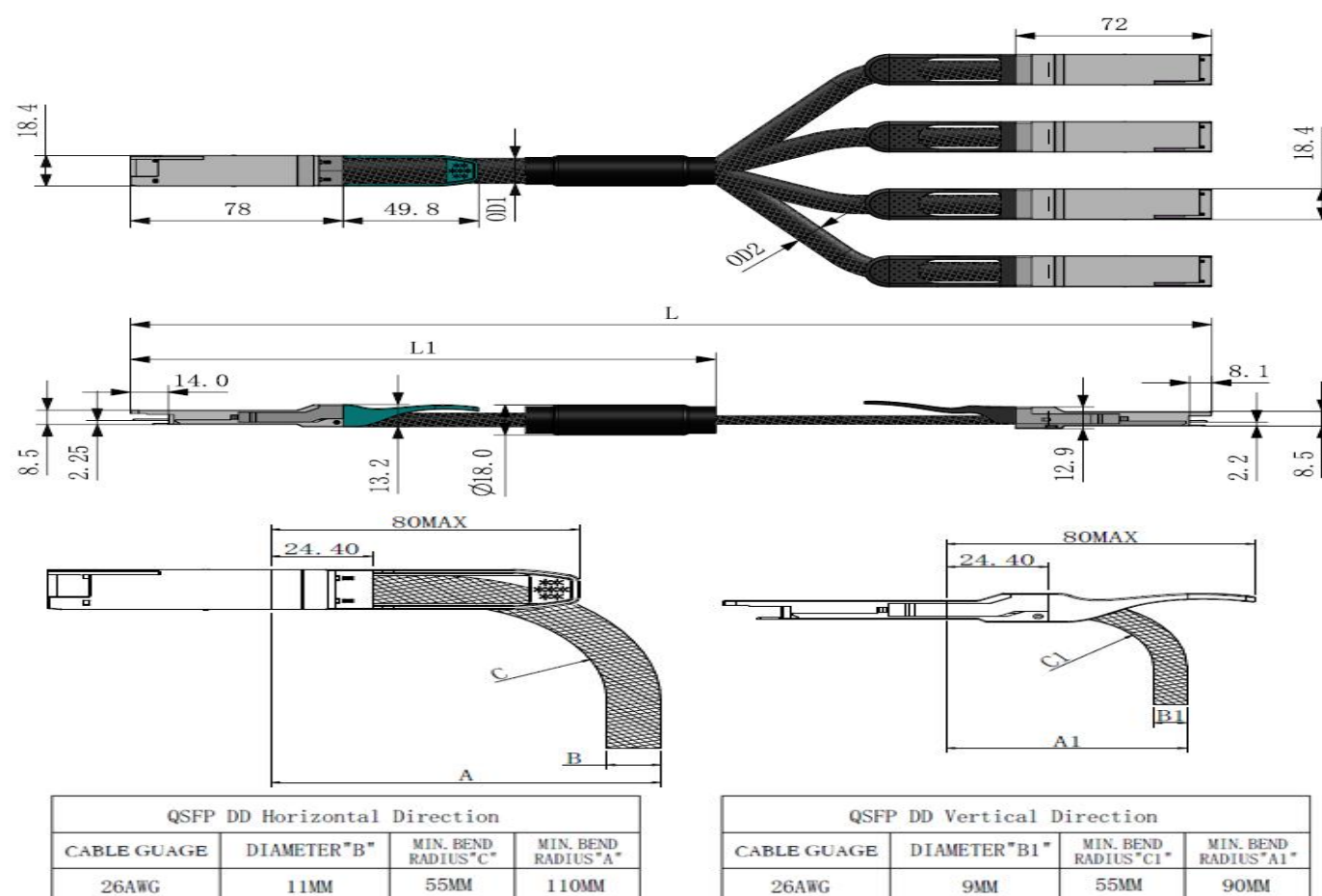
Mechanical Dimensions
