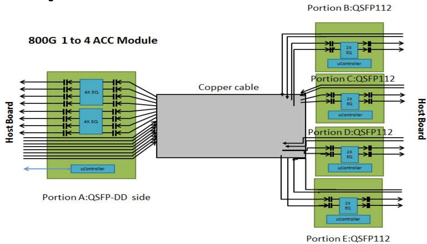
Block Diagram
