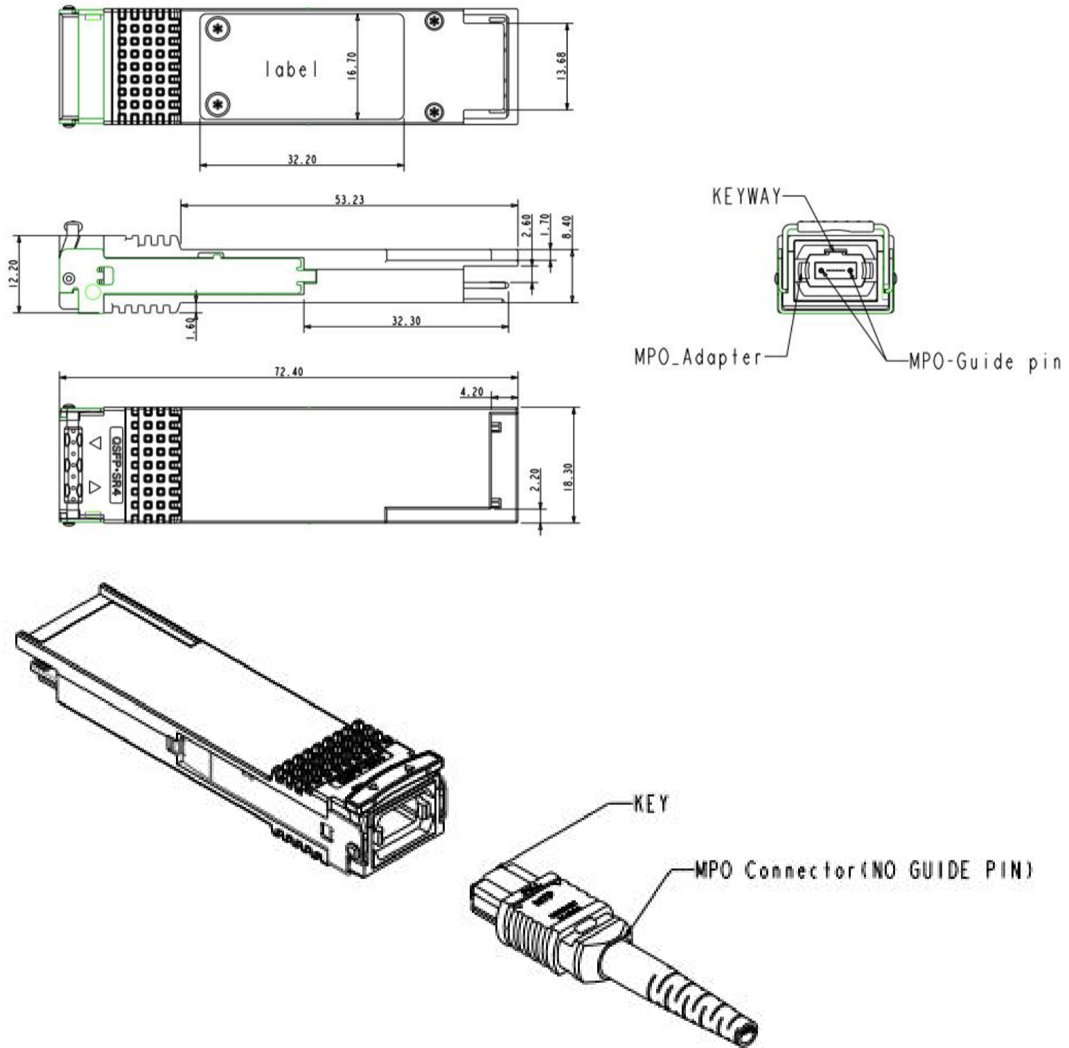
Figure10. Mechanical Specifications
