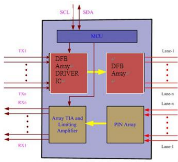
Figure1. Module Block Diagram
