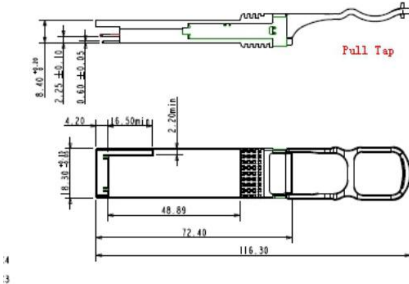
Figure9. Mechanical Specifications
