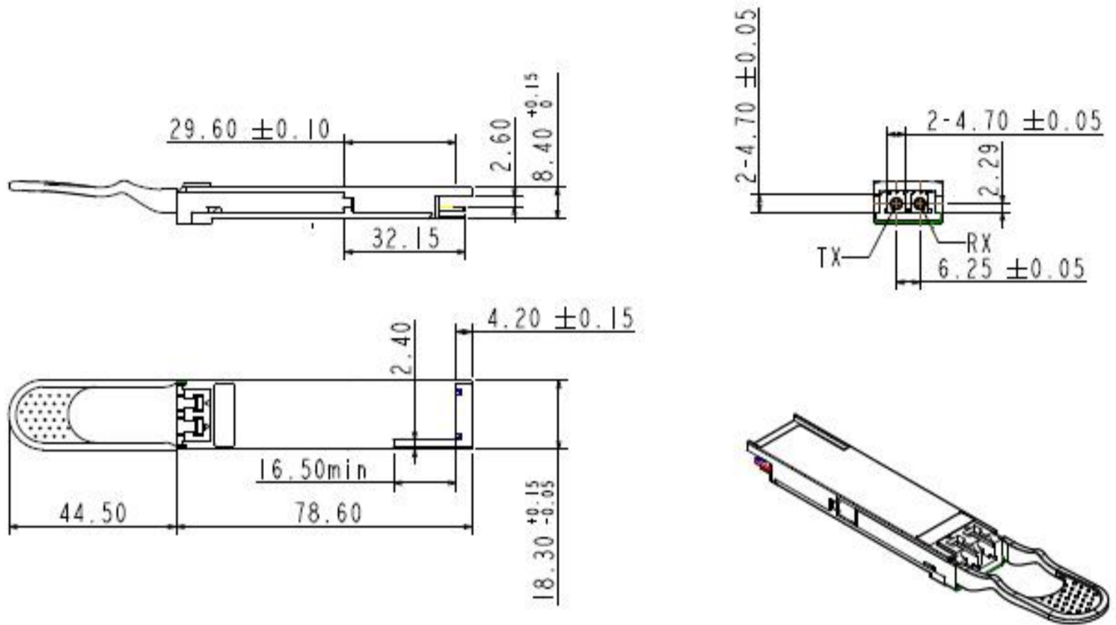
Figure 8. Mechanical Specifications
