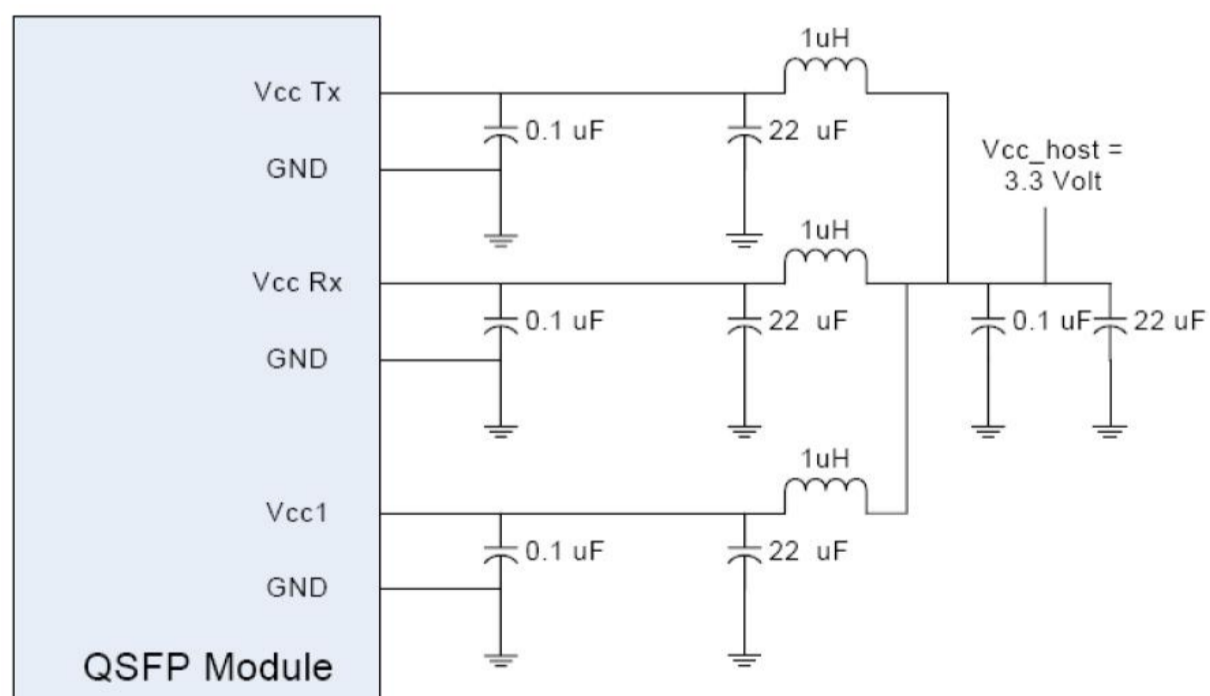
Figure 2. QSFP voltage supply and filtering scheme
