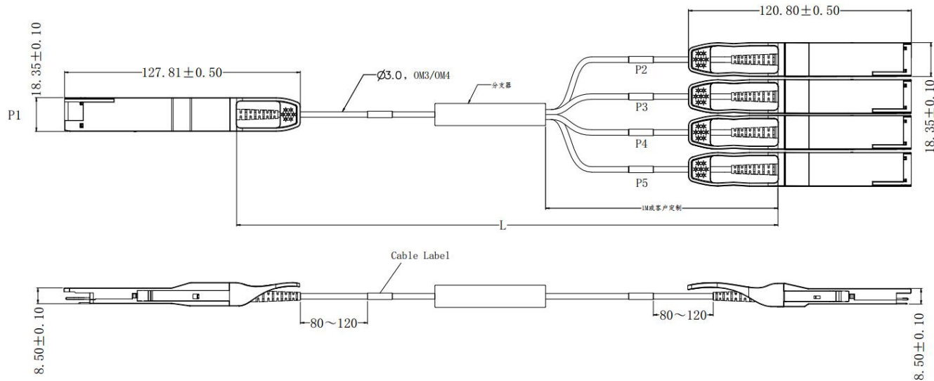
Figure 12. Mechanical Specifications
