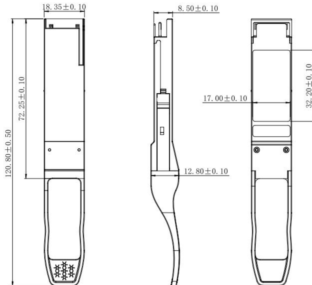
Figure6. Mechanical Specifications
