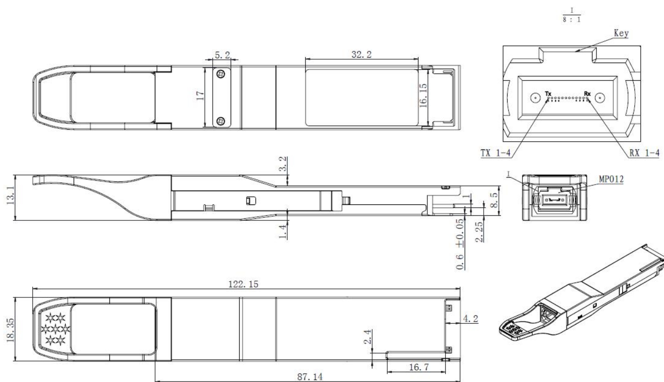
Figure5. Mechanical Specifications
