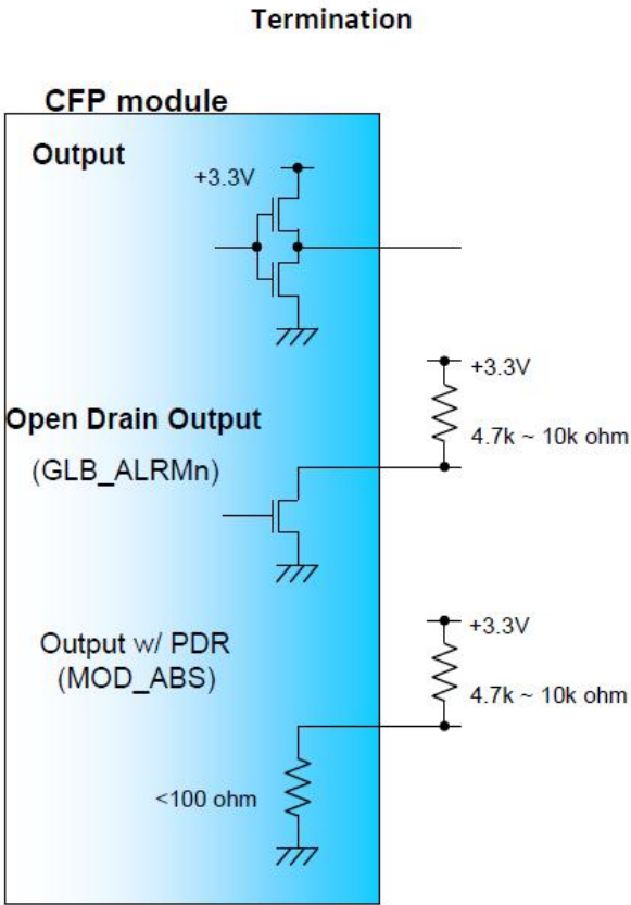
Figure 6 Reference 3.3V LVCMOS Input / Output Termination
