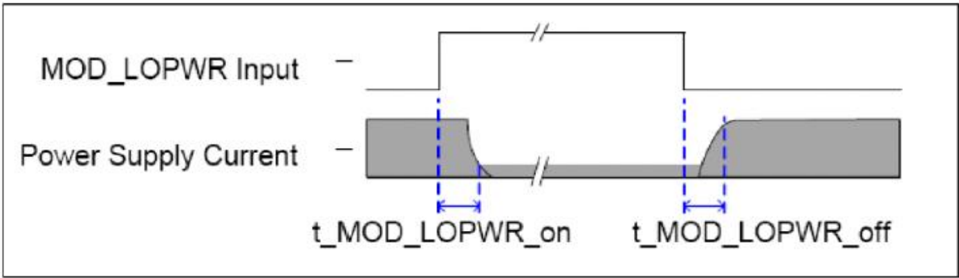
Figure 4 Timing Diagram for MOD_LOPWR
