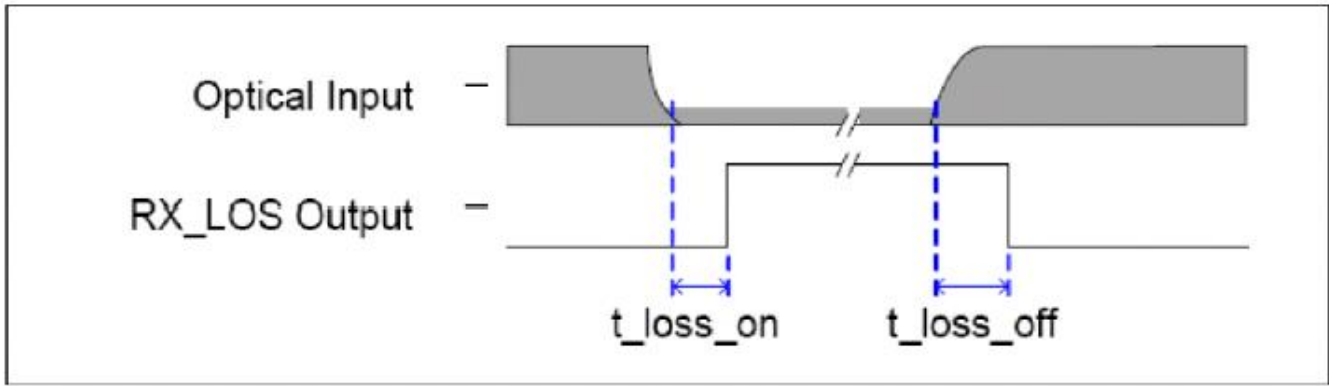
Figure 5 Timing Diagram for RX_LOS
