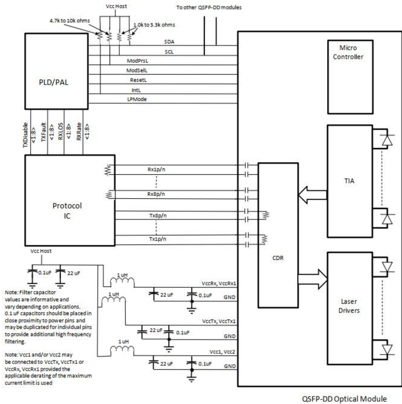
Figure 9 IIC Interface Reference Termination Mode
