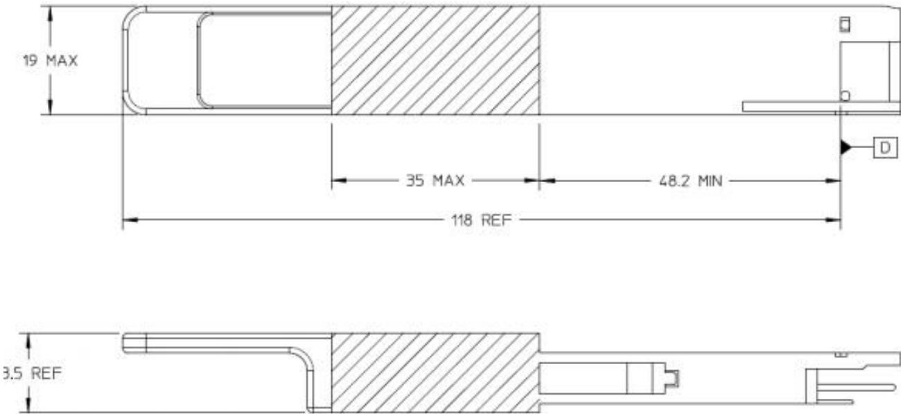
Figure 9 Mechanical Dimensions of the QSFP-DD Optical Module
