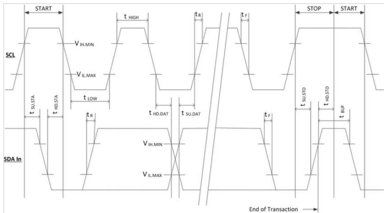
Figure 7 Timing Diagram for the SCL & SDA Pins
