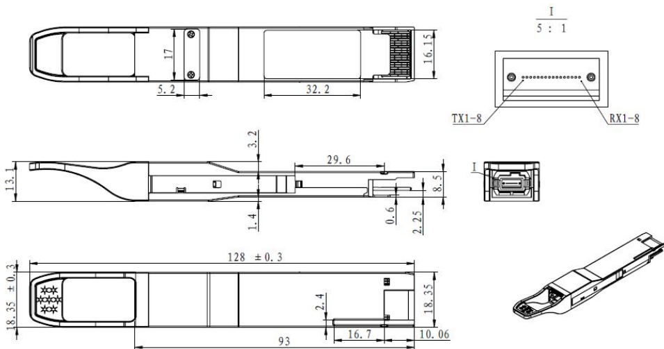
Figure6. Mechanical Specifications
