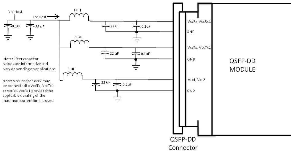
Figure3. Host Board Power Supply Filtering
