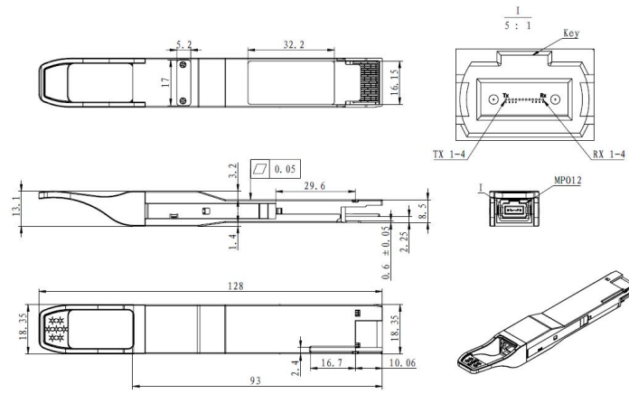
Figure5. Mechanical Specifications
