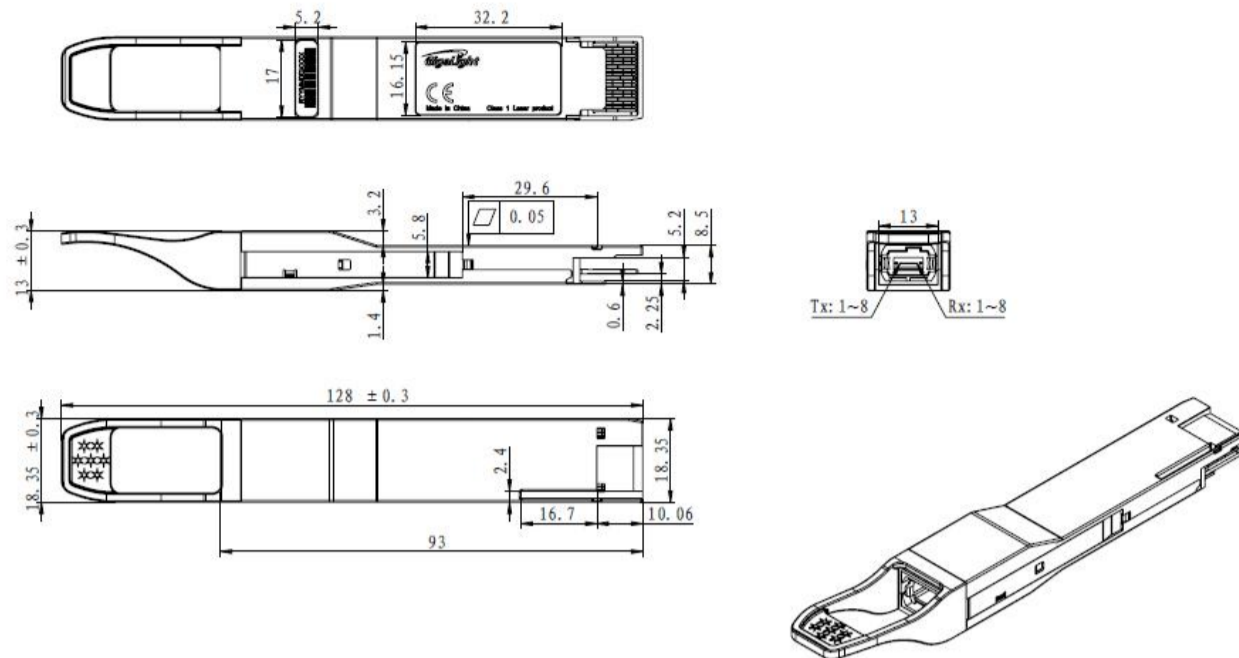
Figure6. Mechanical Specifications
