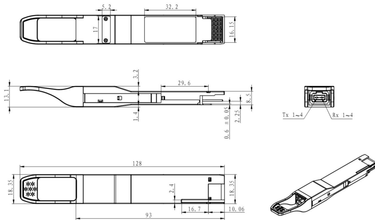
Figure5. Mechanical Specifications
