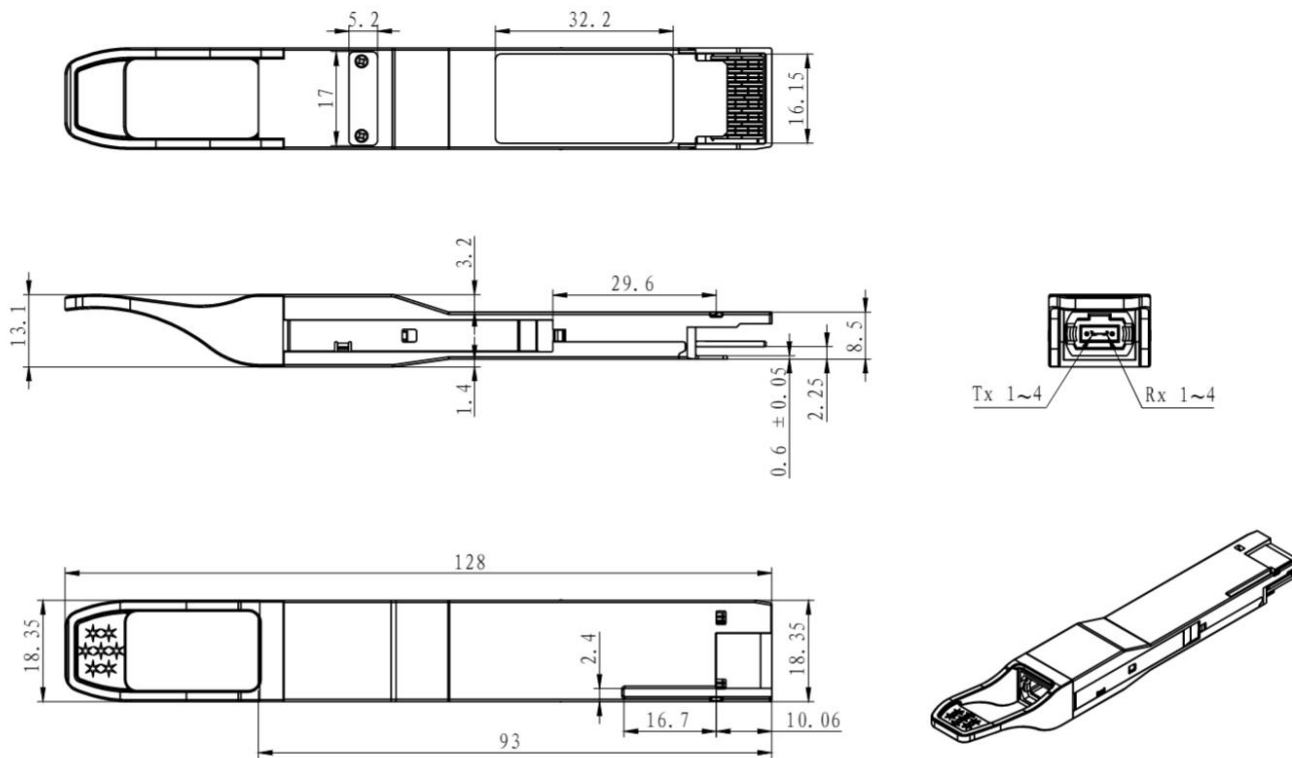
Figure5. Mechanical Specifications
