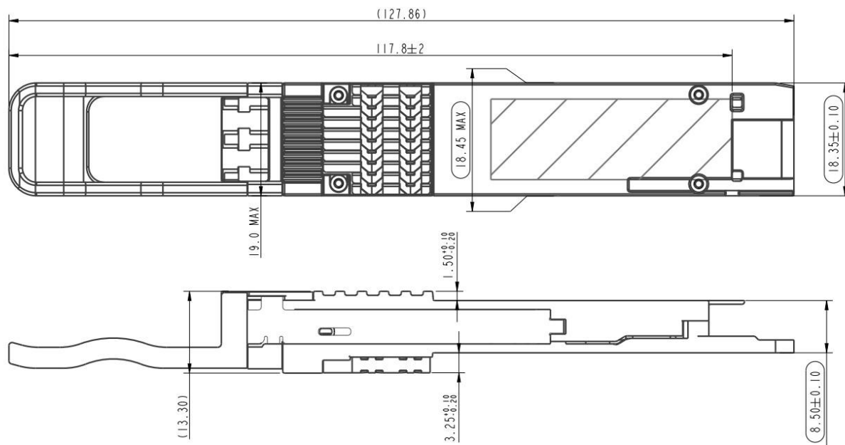
Figure 3. Mechanical Dimensions
