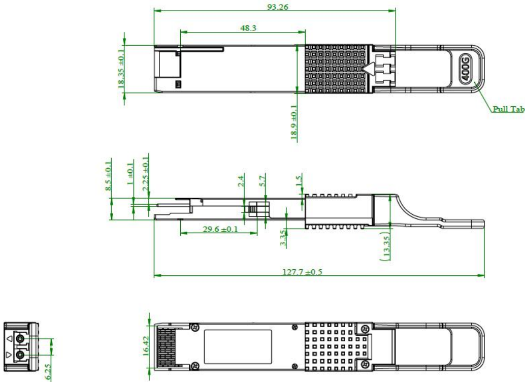
Figure 3. Mechanical Dimensions
