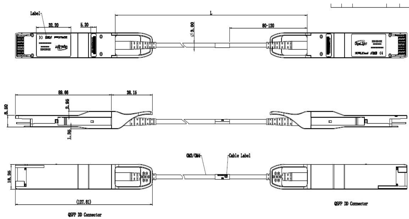
Figure5. Mechanical Specifications
