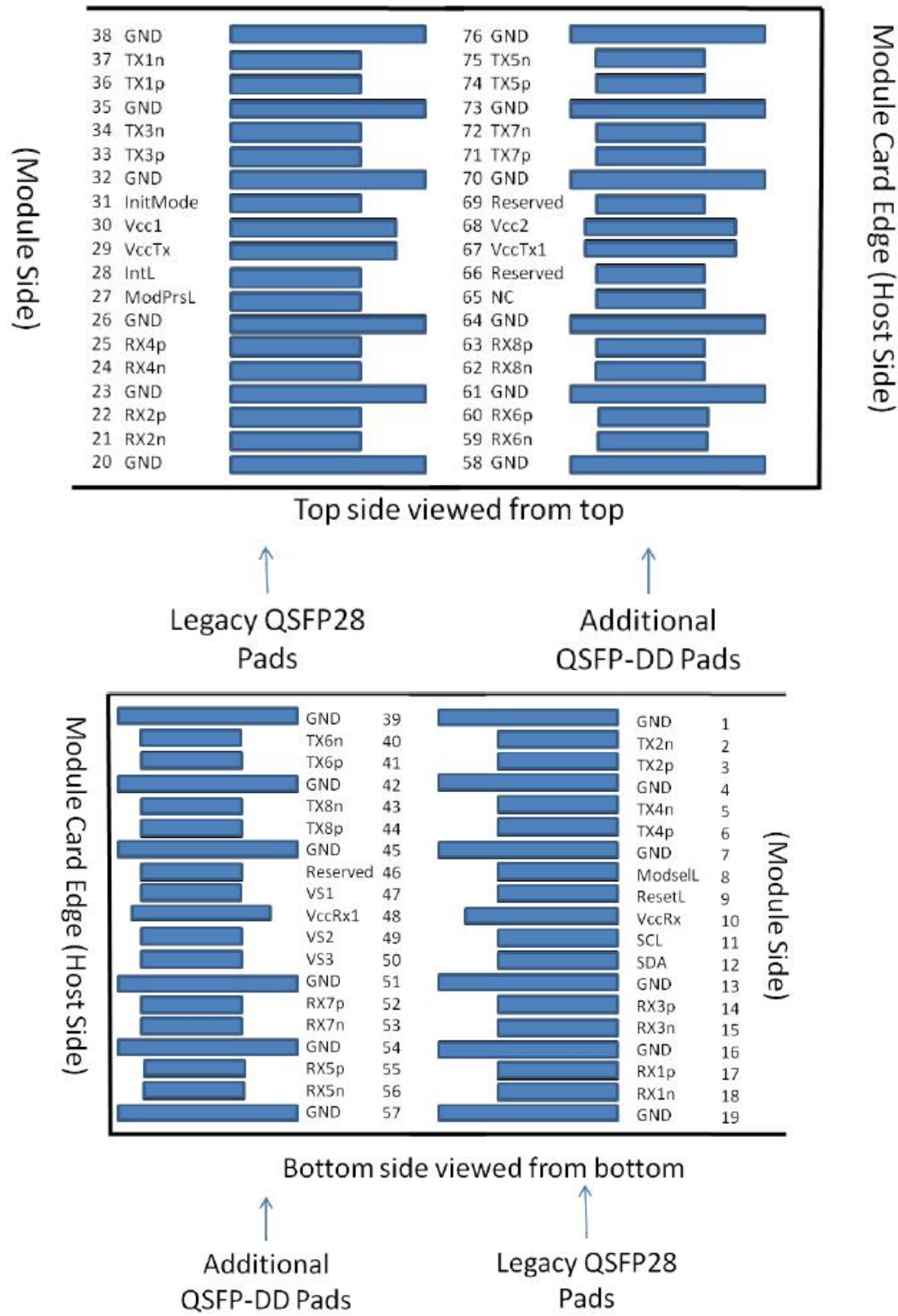
Figure 2. Electrical Pin-out Details
