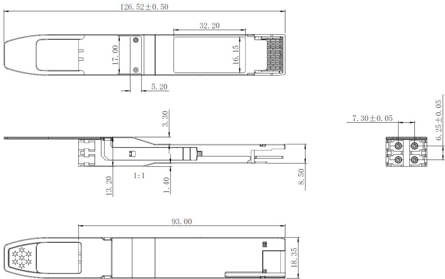
Figure6. Mechanical Specifications
