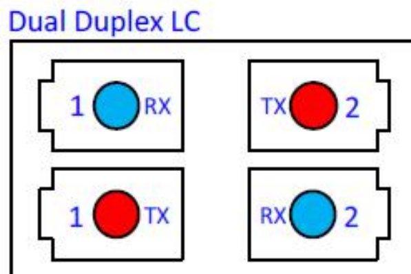
Figure 4. Optical Receptacle
