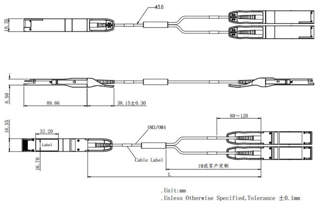
Figure 12. Mechanical Specifications
