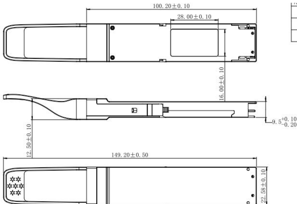
Figure6. Mechanical Specifications
