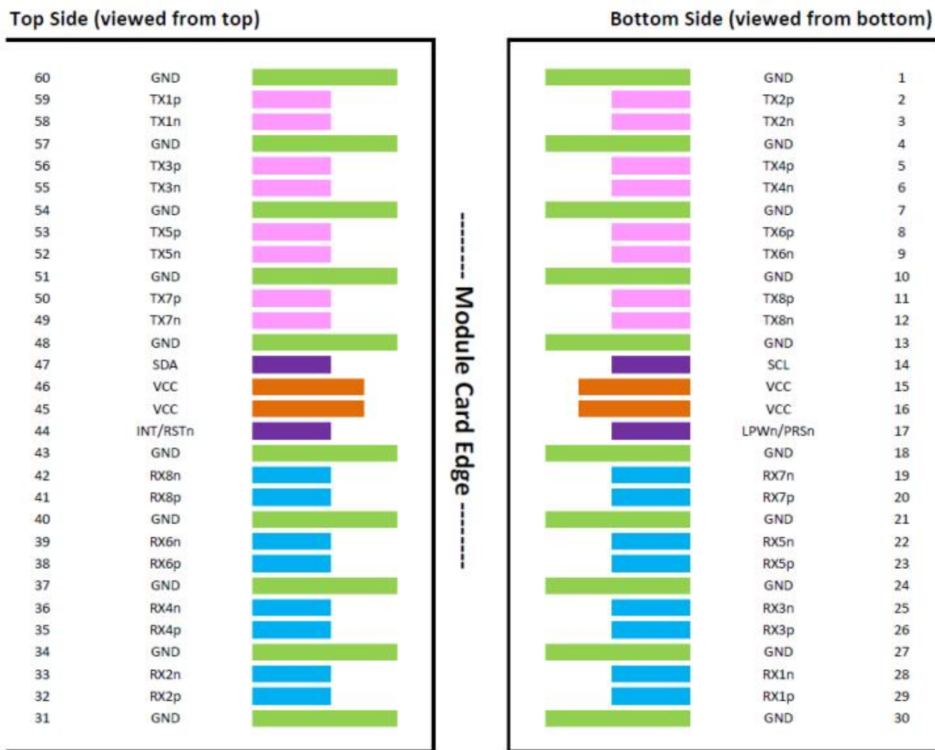
Figure2. Electrical Pin-out Details
