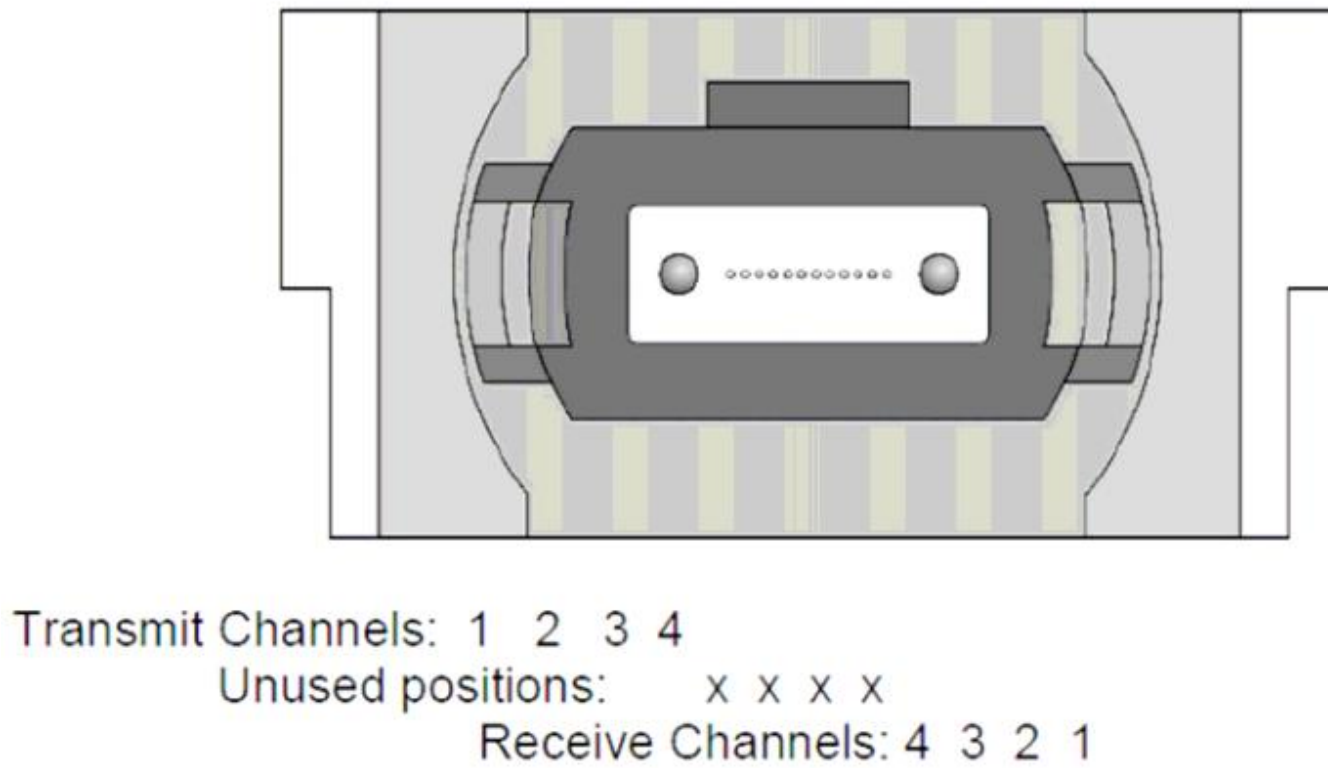
Figure 4. Optical Receptacle and Channel Orientation
