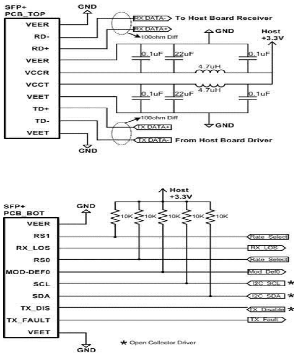
Figure 3. Recommended Interface Circuit
