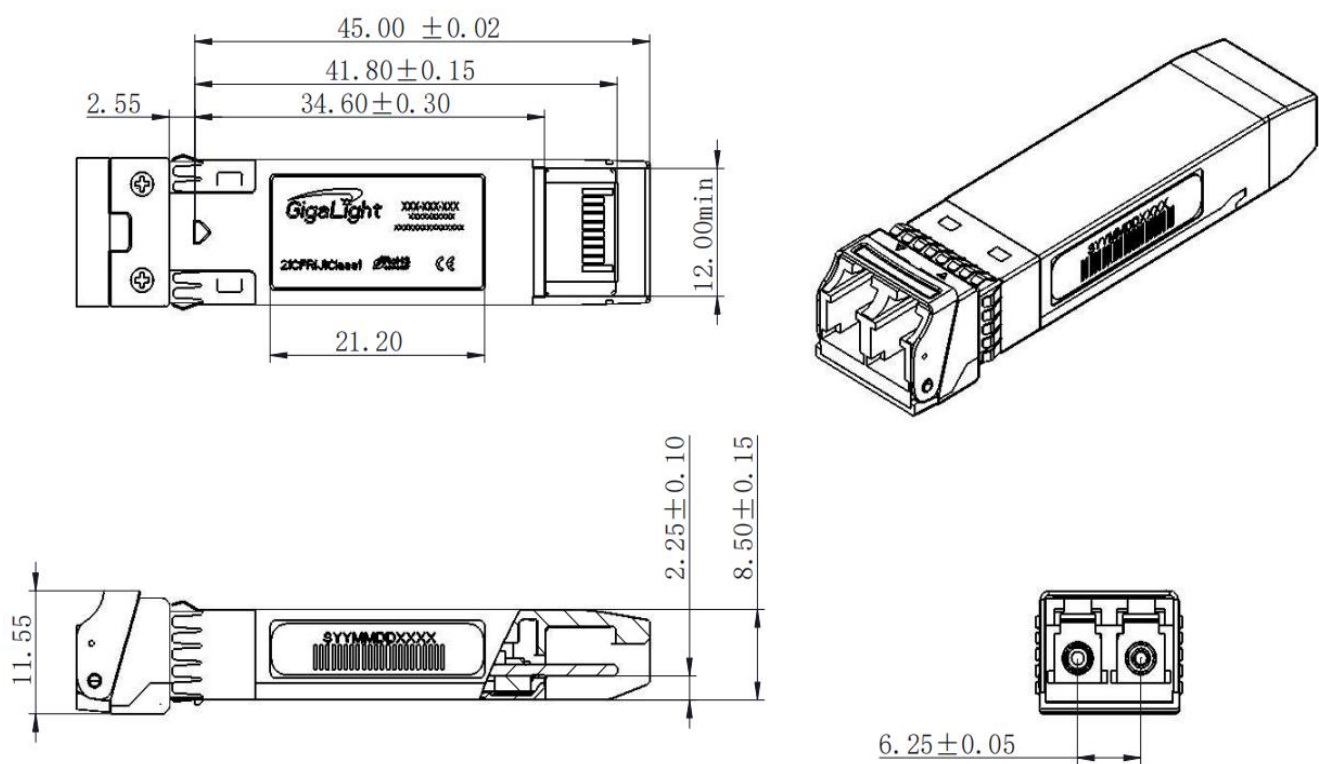
Figure 5. Mechanical Specifications
