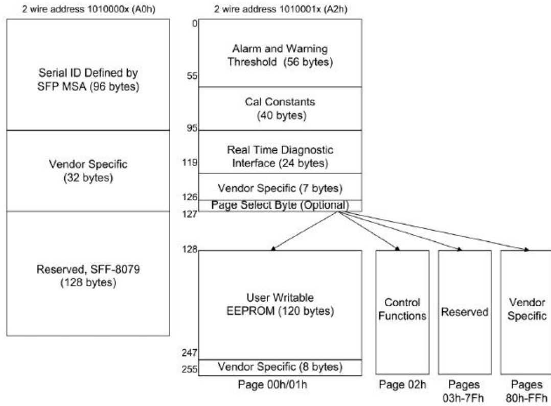
Figure 5. SFP28 Memory Map
