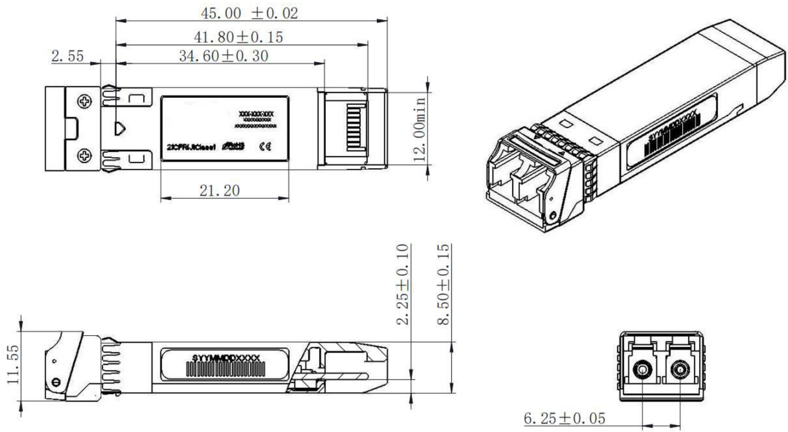
Figure 7. Mechanical Specifications
