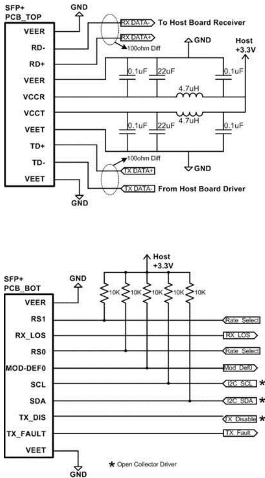
Figure 4. Recommended Interface Circuit
