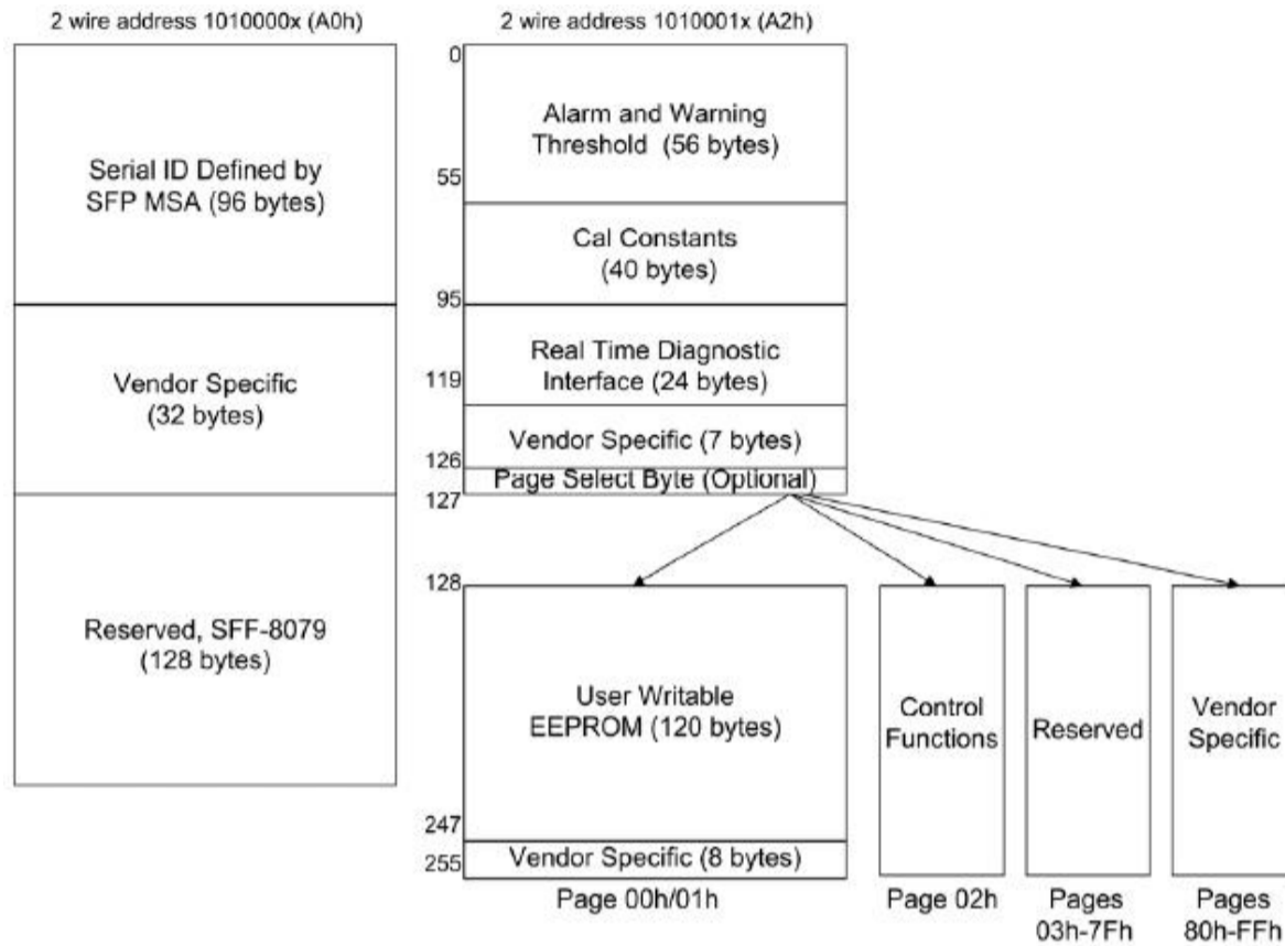
Figure 5. SFP28 Memory Map
