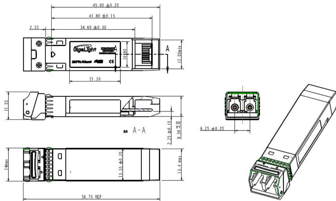
Figure 6. Mechanical Specifications
