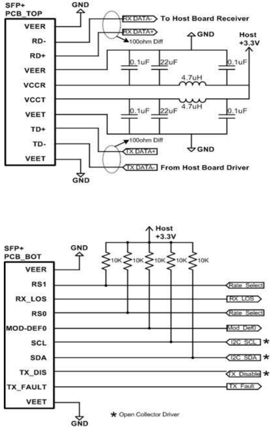
Figure 3. Recommended Interface Circuit
