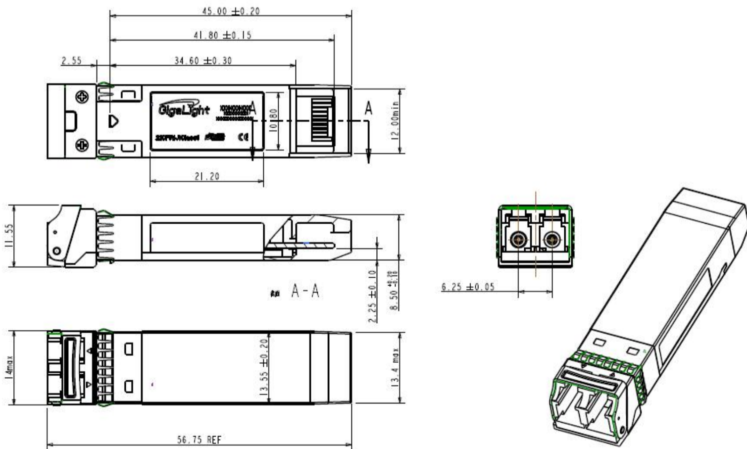
Figure 4. Mechanical Specifications
