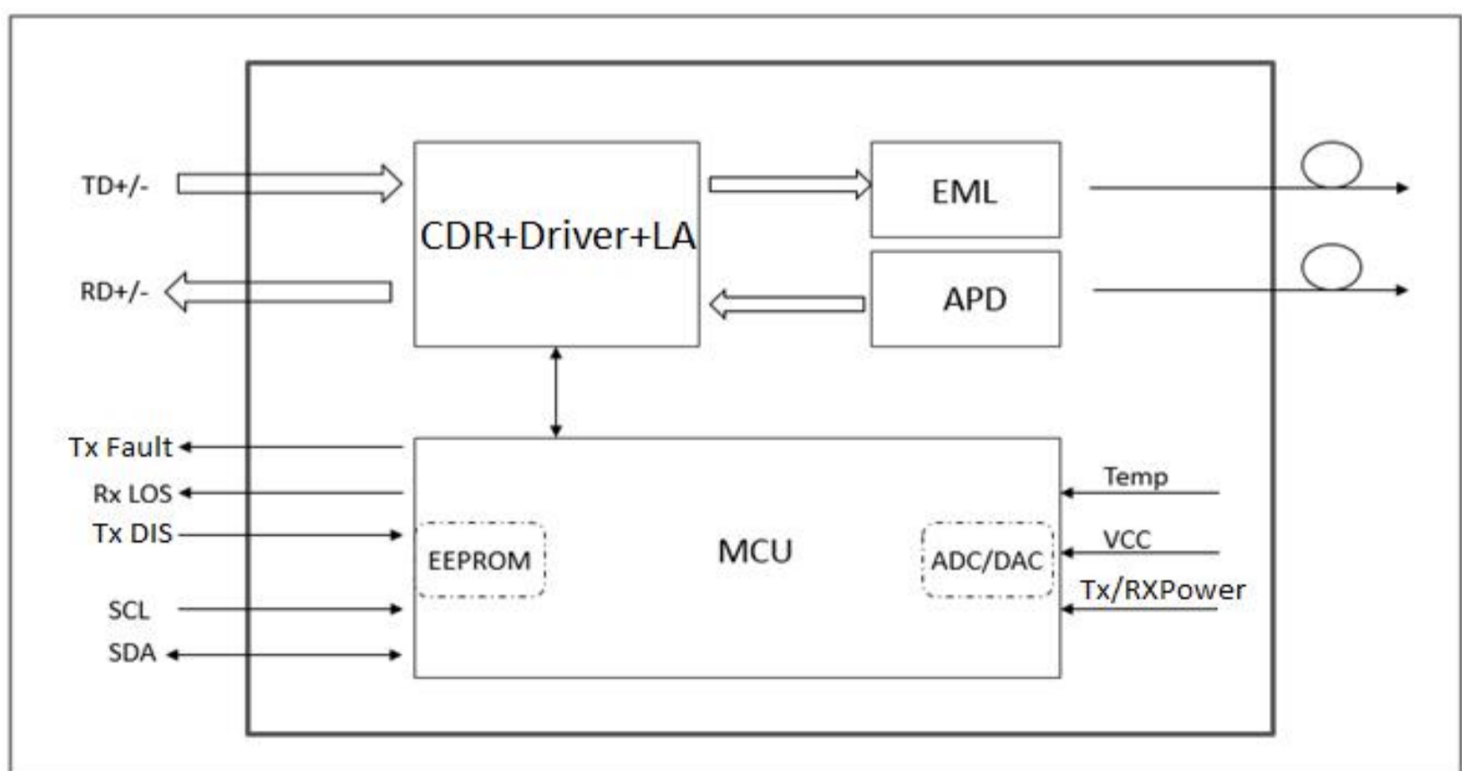
Figure 1. Module Block Diagram
