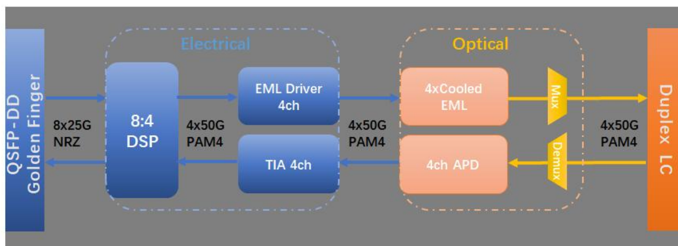
Figure1. Module Block Diagram
