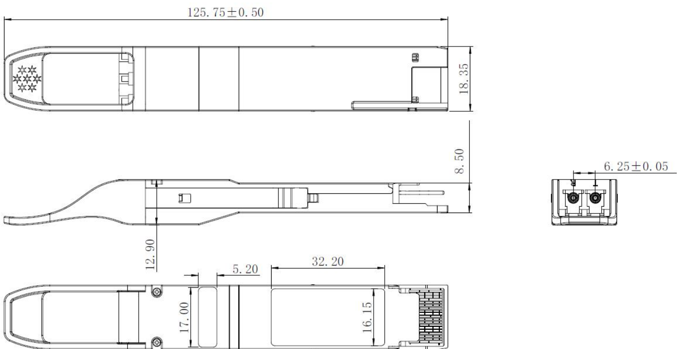
Figure6. Mechanical Specifications
