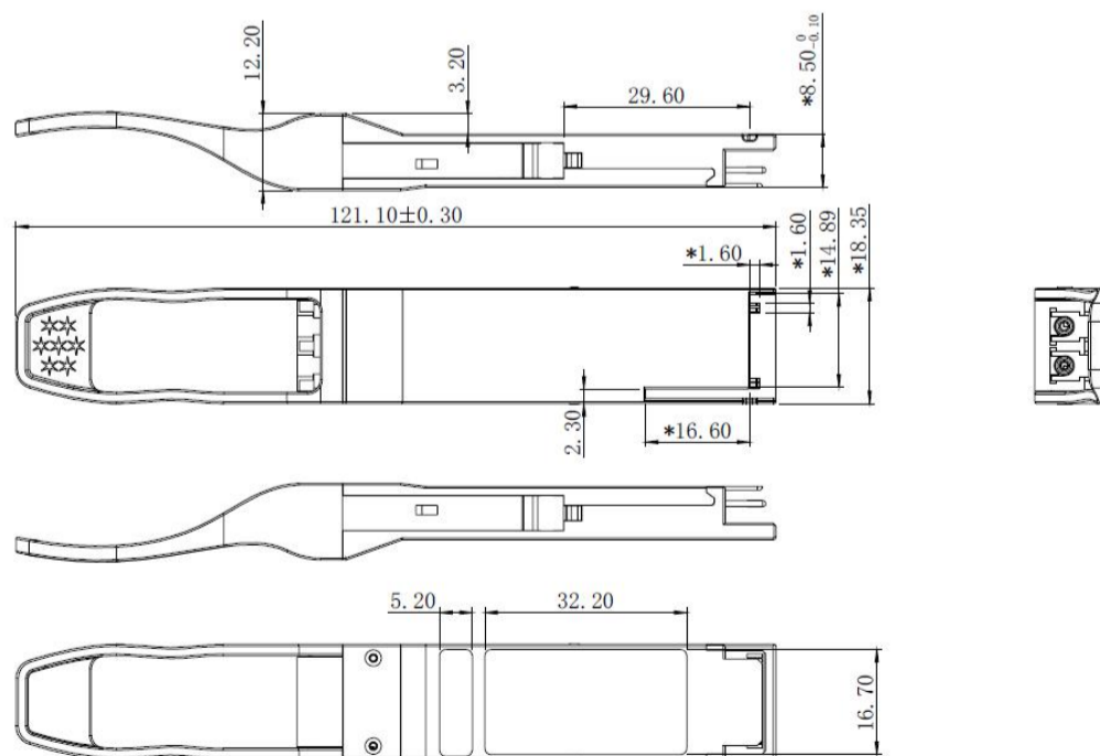
Figure 12. Mechanical Specifications
