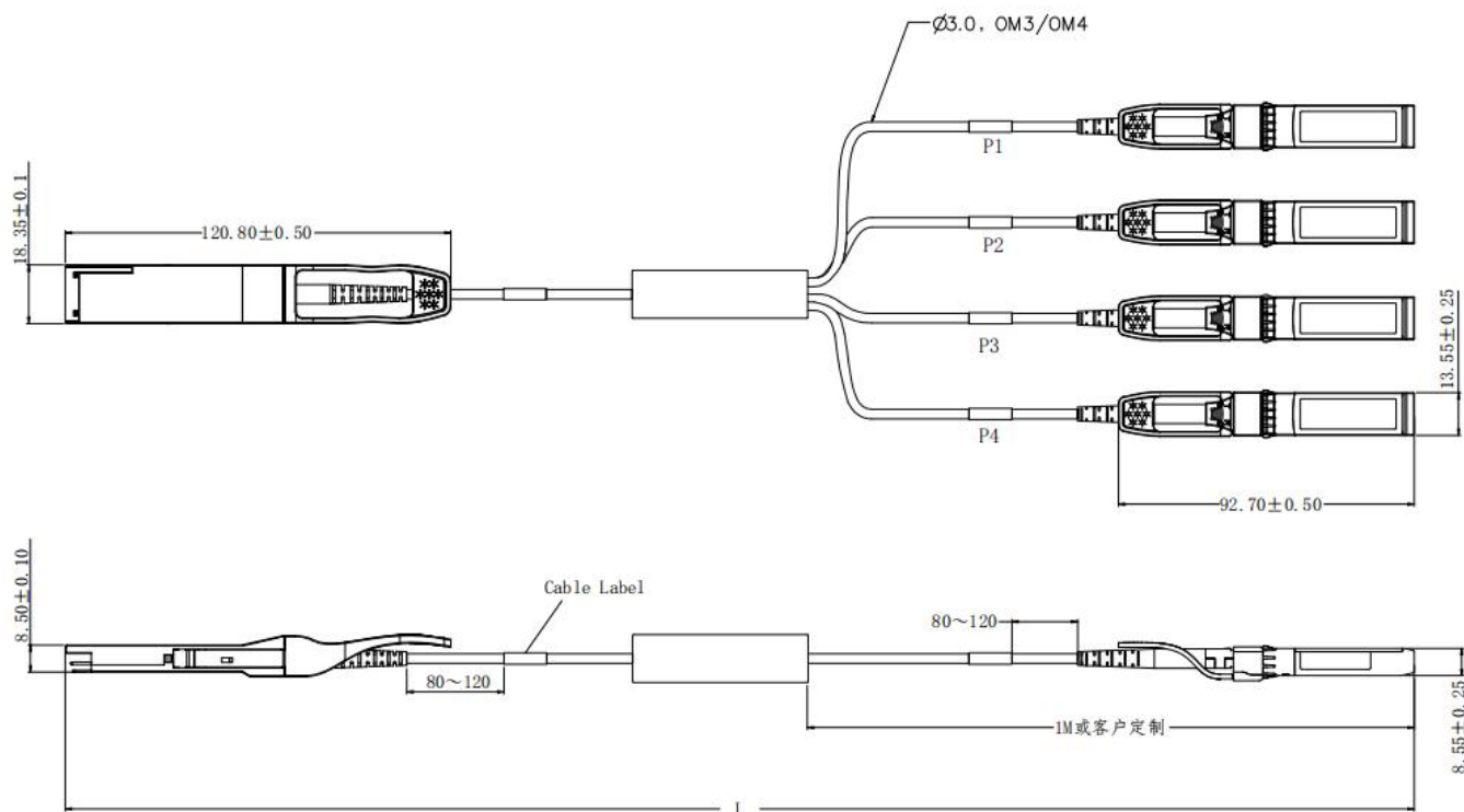
Figure 12. Mechanical Specifications
