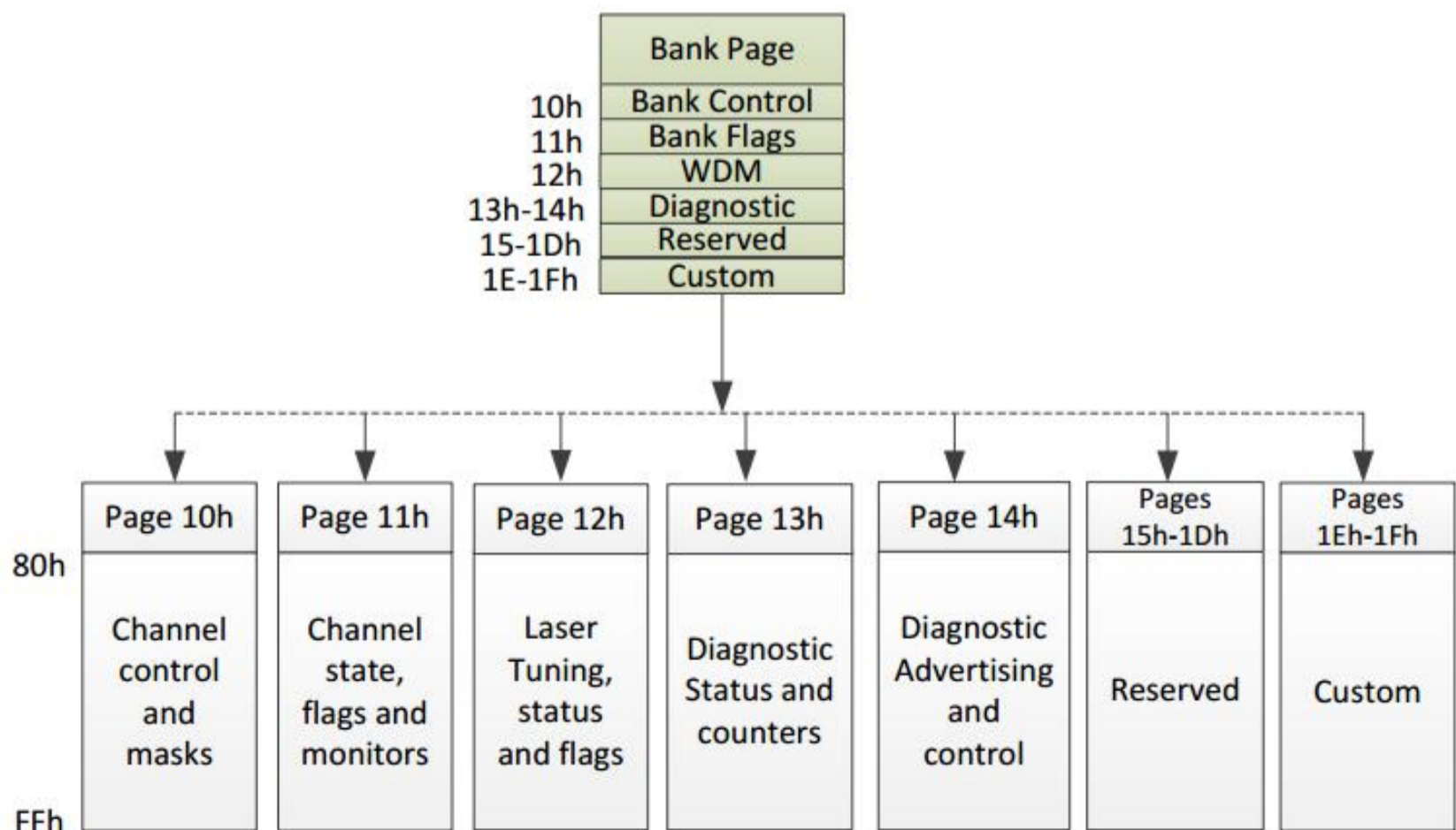
Figure 5. Additional Supported Bank Page Memory Map
