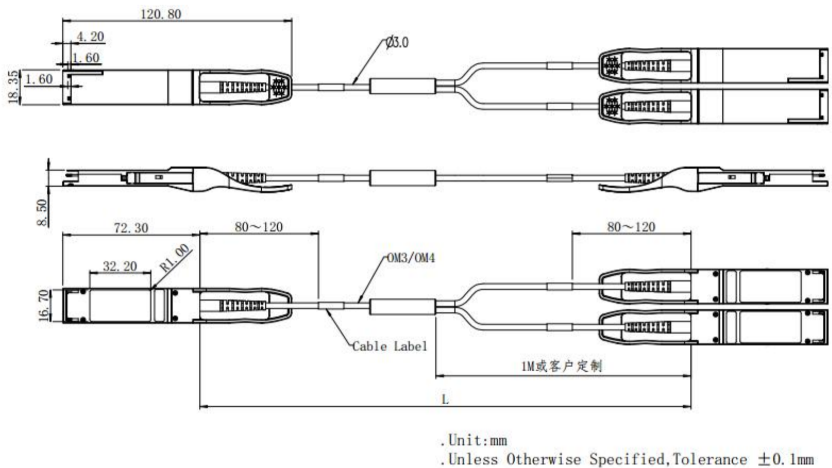
Figure 12. Mechanical Specifications
