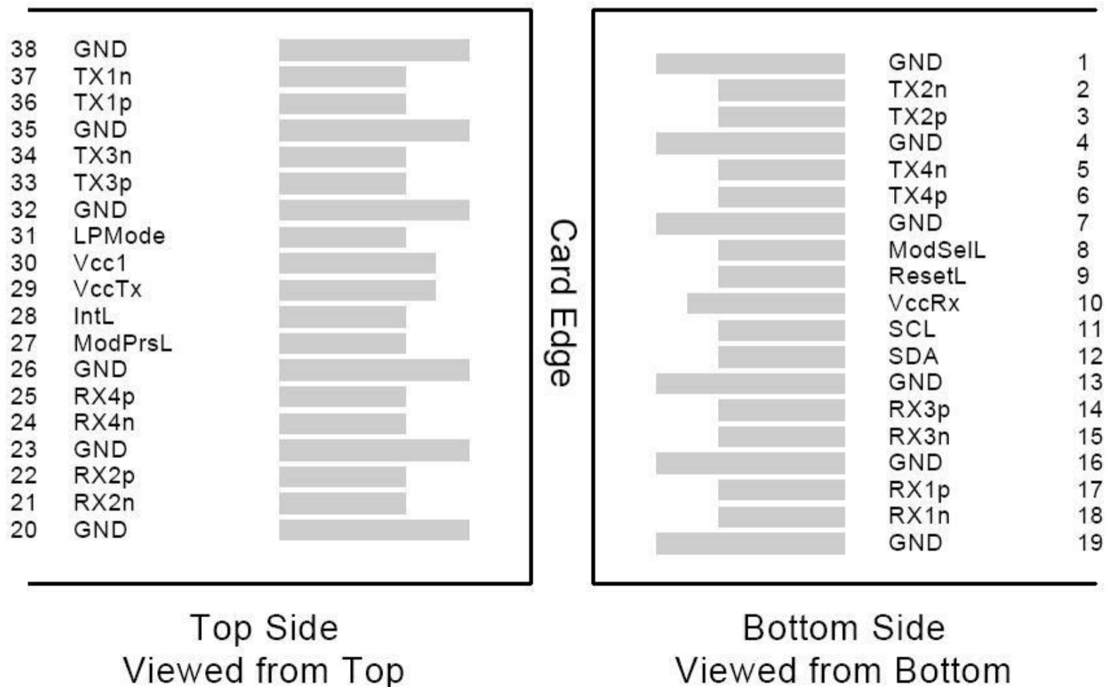
Figure 2. Electrical Pin-out Details
