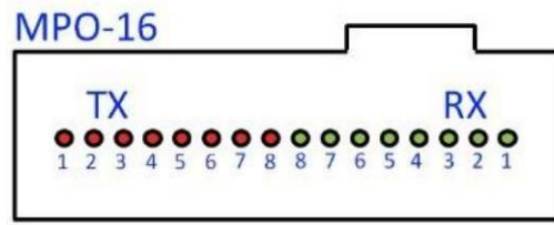
Figure 4. Optical Receptacle and Channel Orientation
