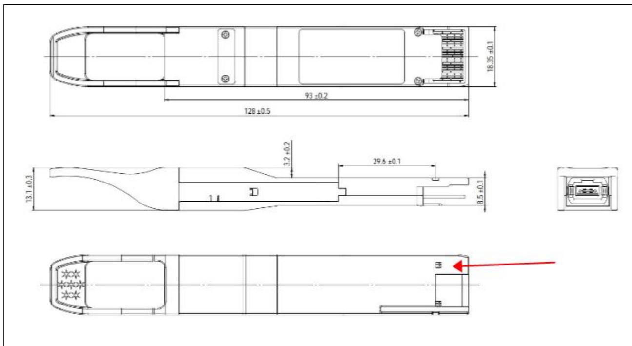
Figure10. Mechanical Specifications
