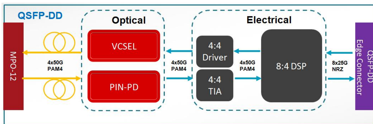
Figure1. Module Block Diagram
