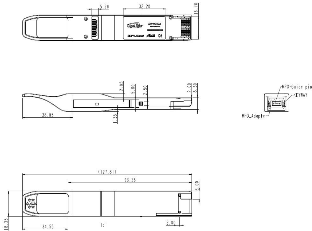
Figure6. Mechanical Specifications
