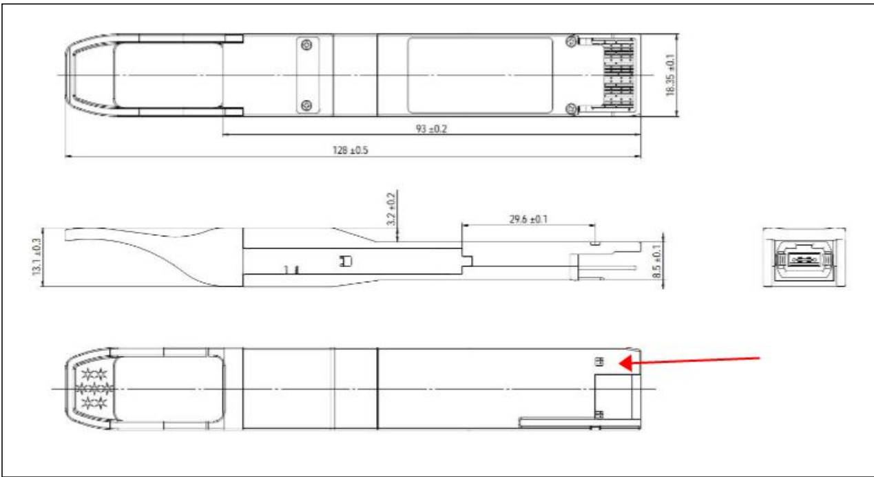
Figure10. Mechanical Specifications
