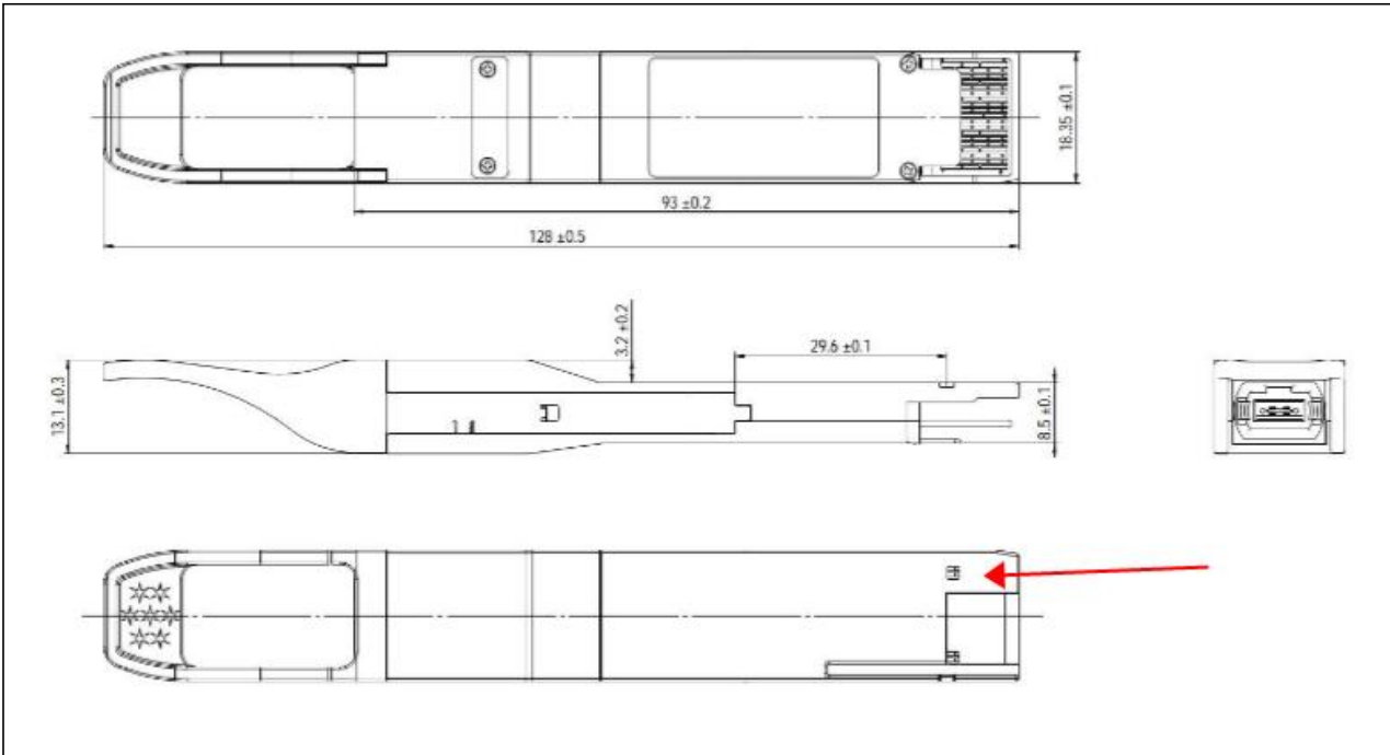
Figure9. Mechanical Specifications
