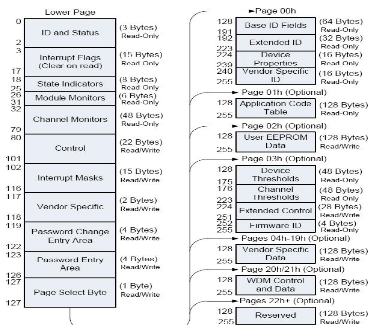
Figure 5. QSFP28 Memory Map
