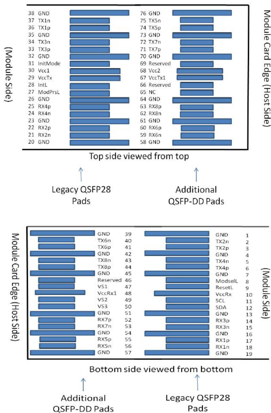
Figure 2. Electrical Pin-out Details
