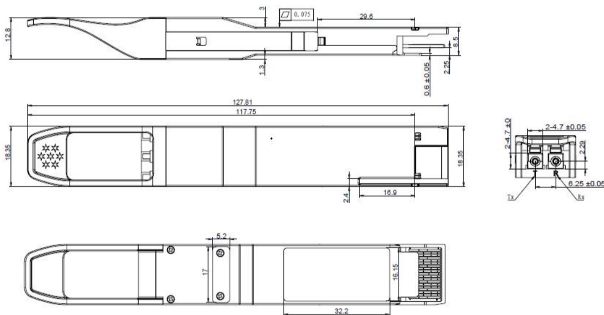
Figure5. Mechanical Specifications
