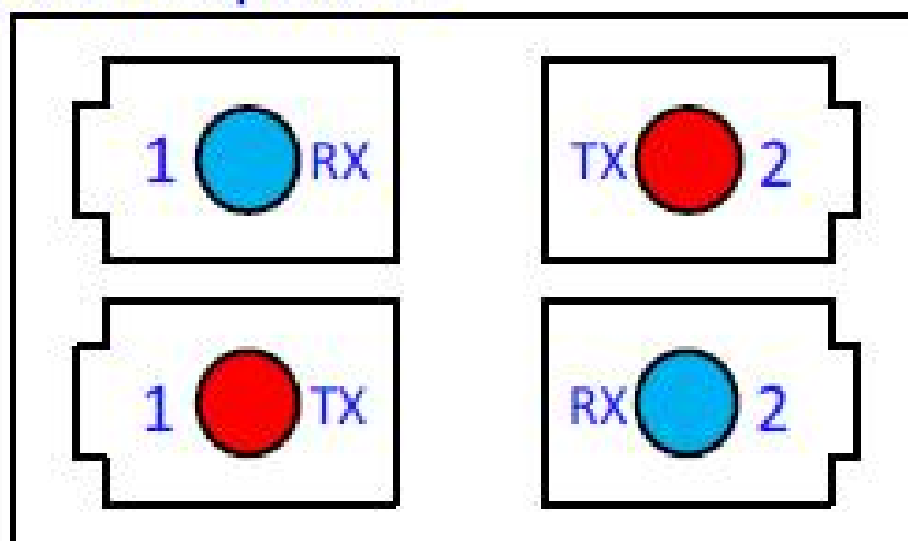
Figure 4. Optical Receptacle
