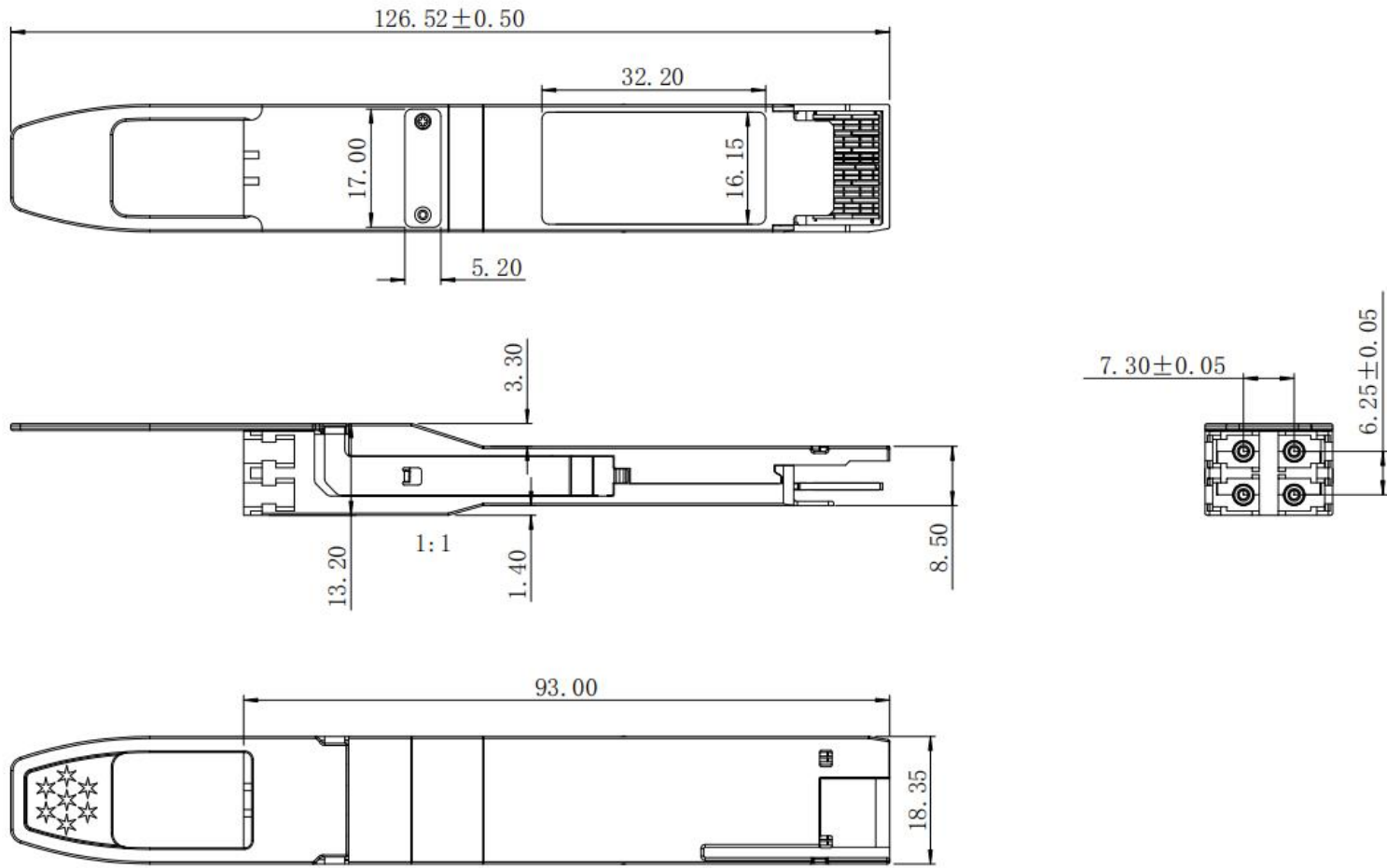
Figure6. Mechanical Specifications
