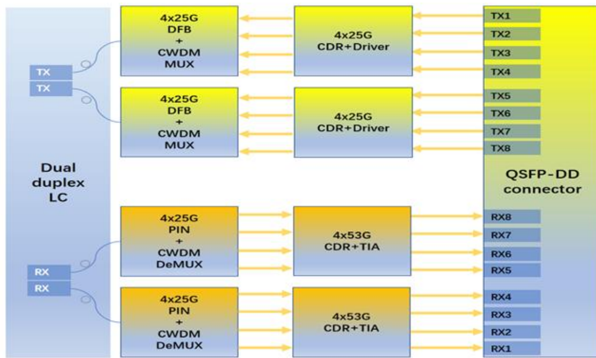
Figure1. Module Block Diagram
