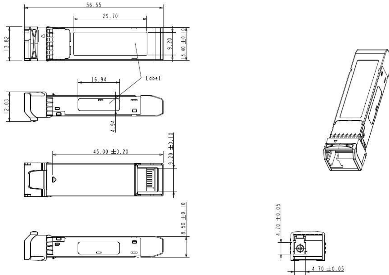
Figure 3. Mechanical Specifications
